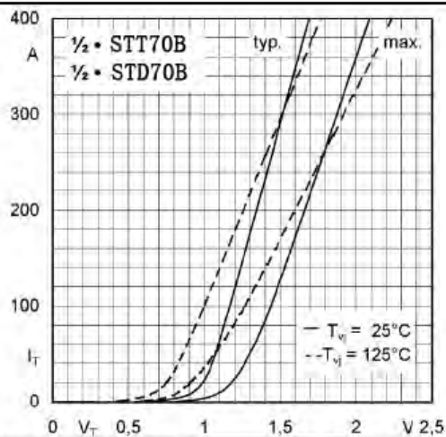
Fig. 7 On-state characteristics
