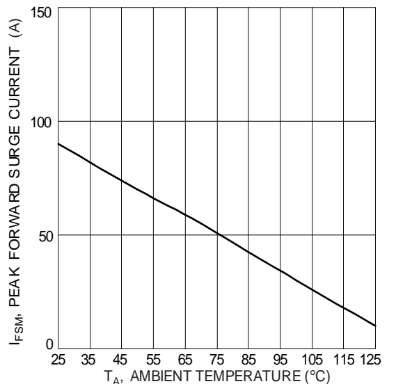
Fig. 6 Non-Repetitive Forward Surge Current Derating Curve
