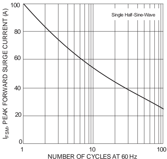
Fig. 5 Max Non-Repetitive Peak Fwd Surge Current
