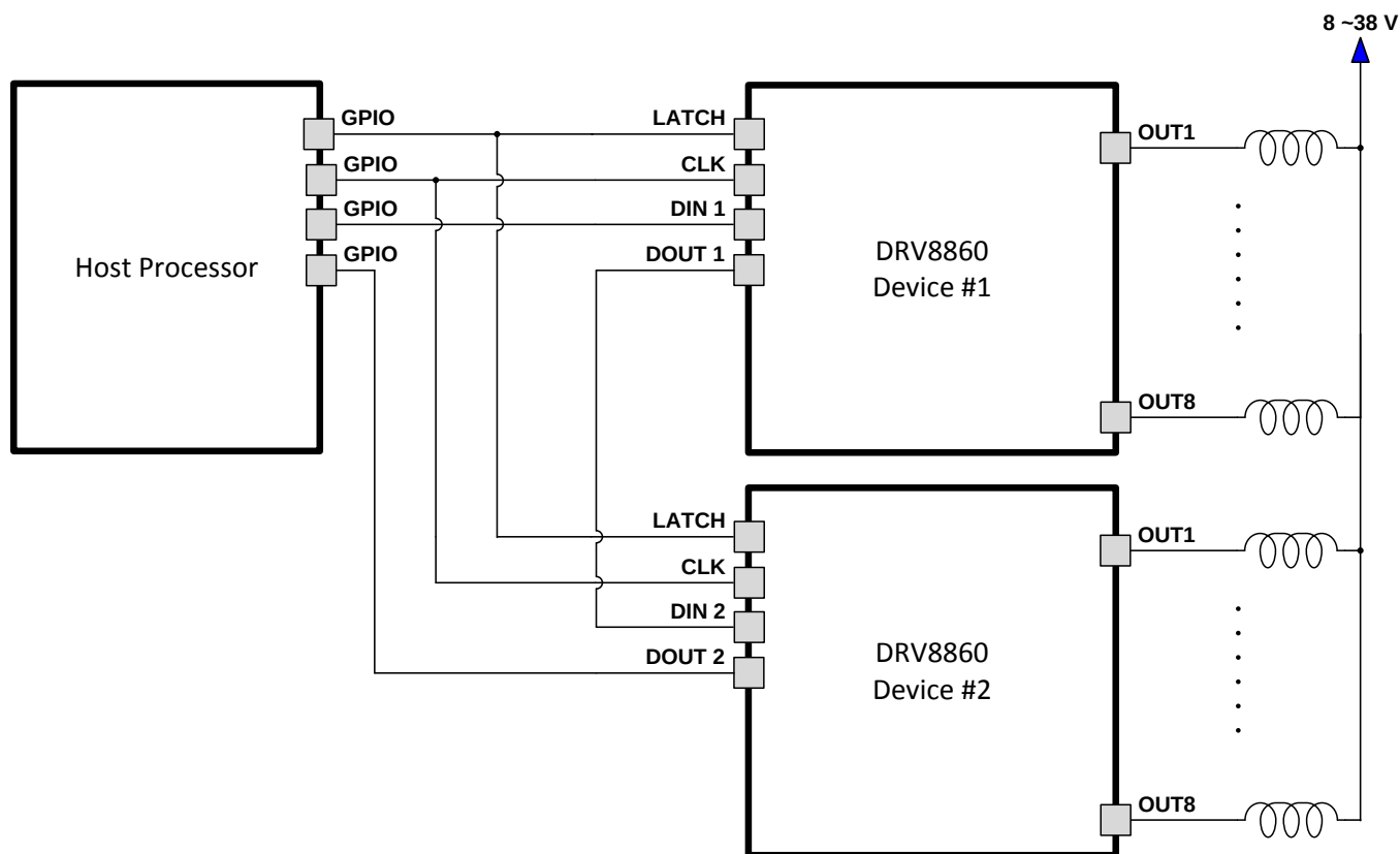
Figure 8. Daisy-Chain Connection
