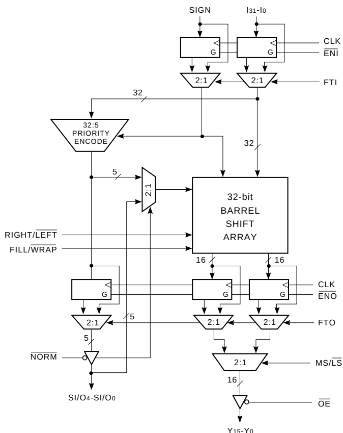
LSH33 BLOCK DIAGRAM
