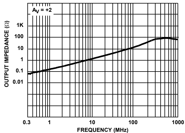
FIGURE 20. OUTPUT IMPEDANCE
