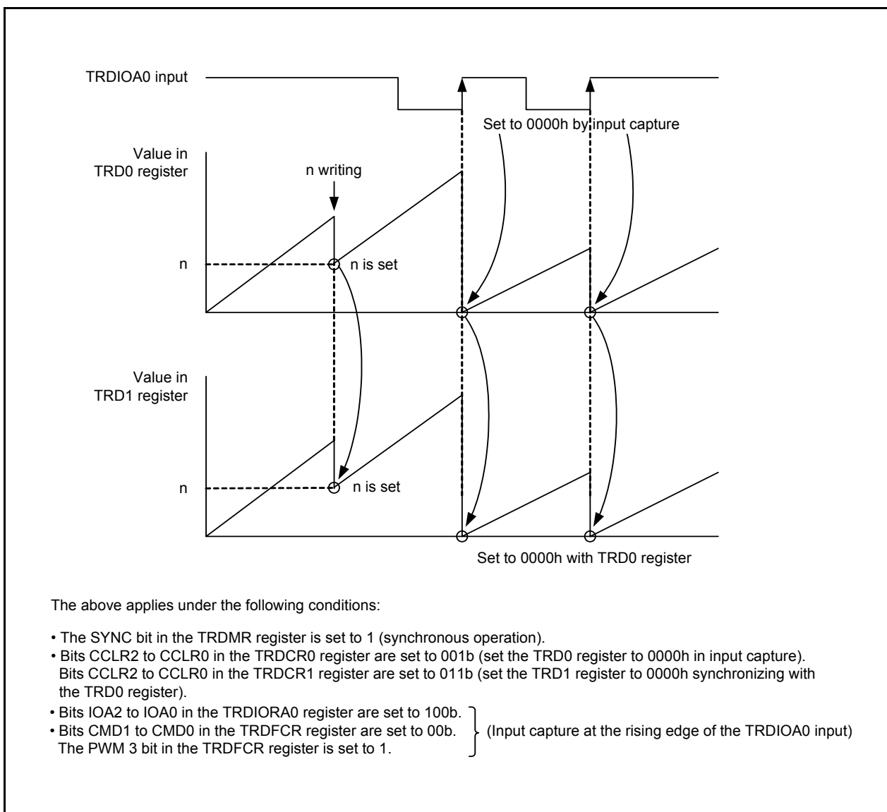
Figure 14.66 Synchronous Operation
