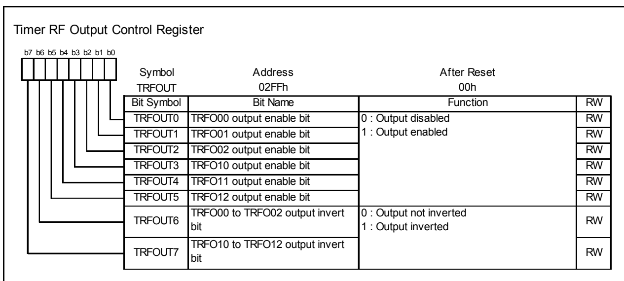
Figure 14.180 TRFOUT Register
