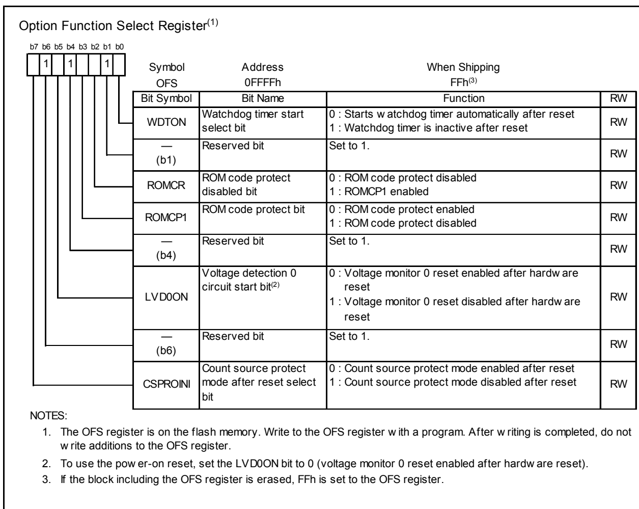
Figure 5.4 OFS Register
