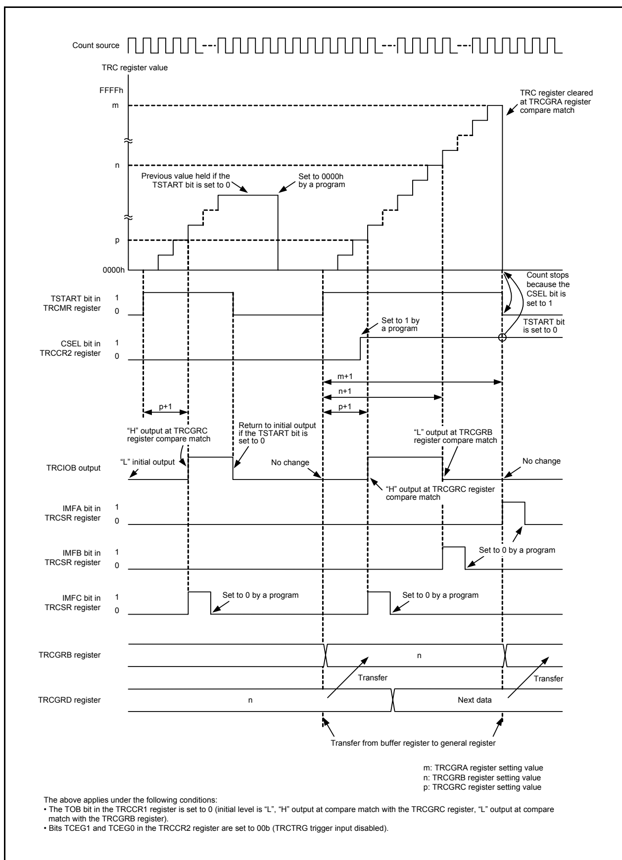
Figure 14.58 Operating Example of PWM2 Mode (TRCTRГ Trigger Input Disabled)
