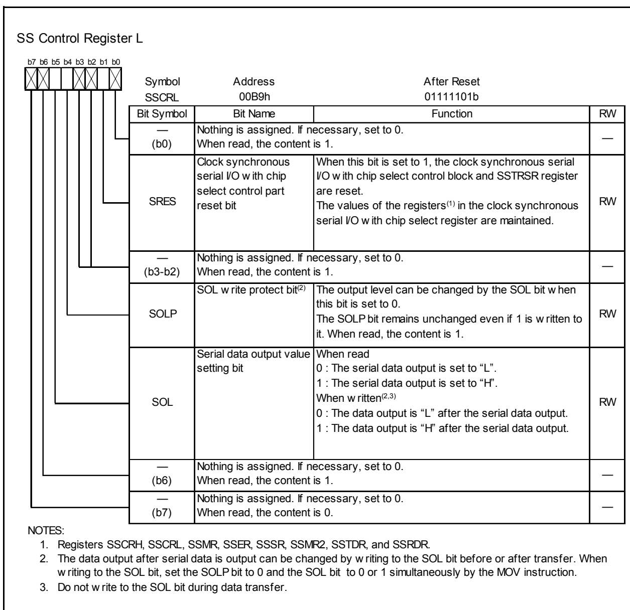
Figure 16.4 SSCRL Register
