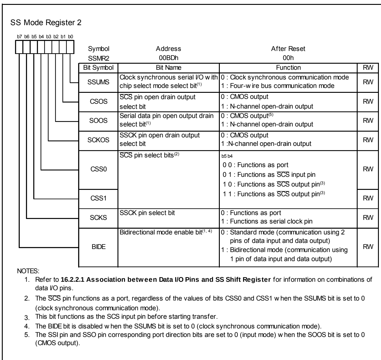
Figure 16.8 SSMR2 Register
