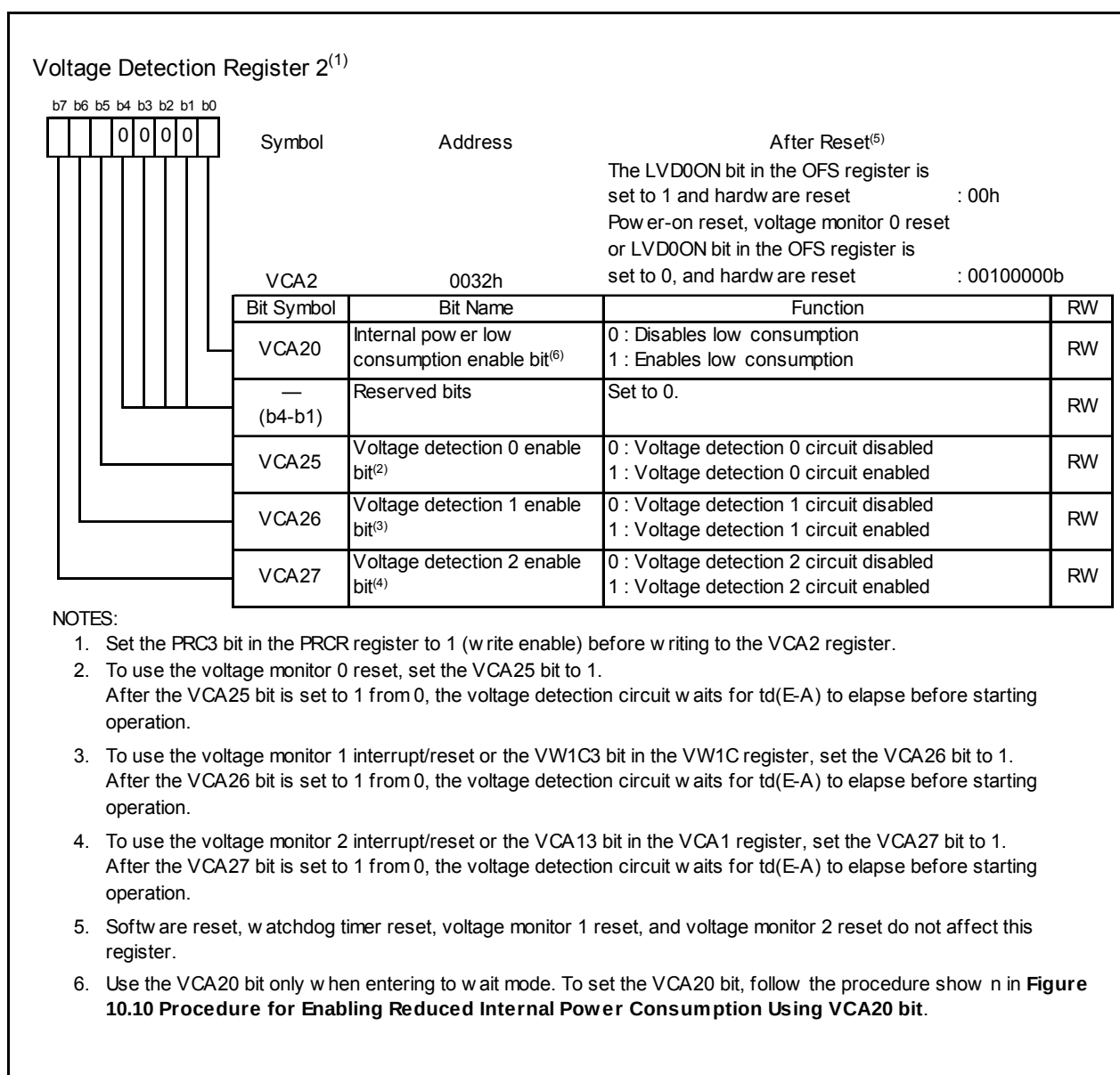
Figure 10.9 VCA2 Register
