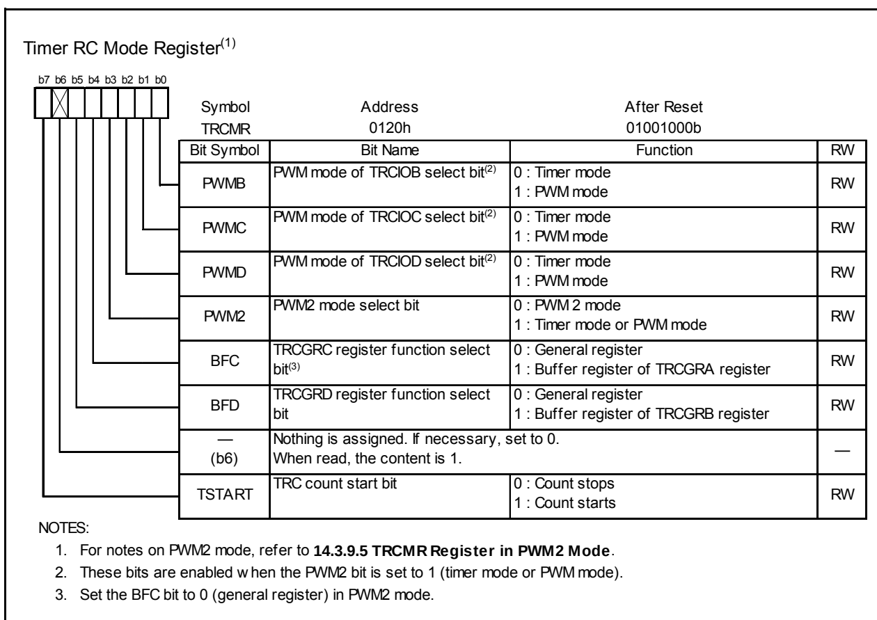
Figure 14.28 TRCMR Register
