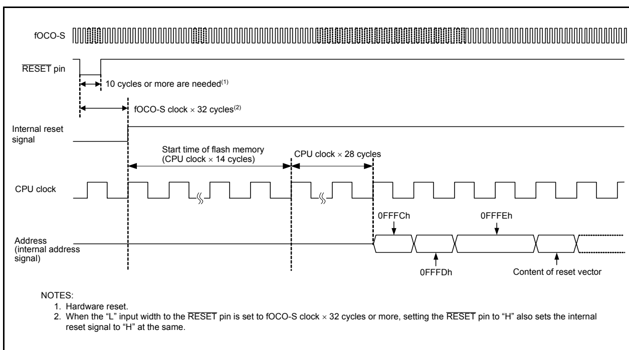
Figure 5.3 Reset Sequence
