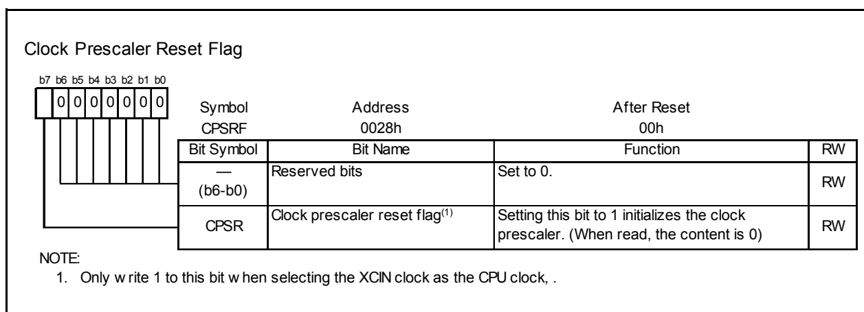
Figure 10.8 CPSRF Register
