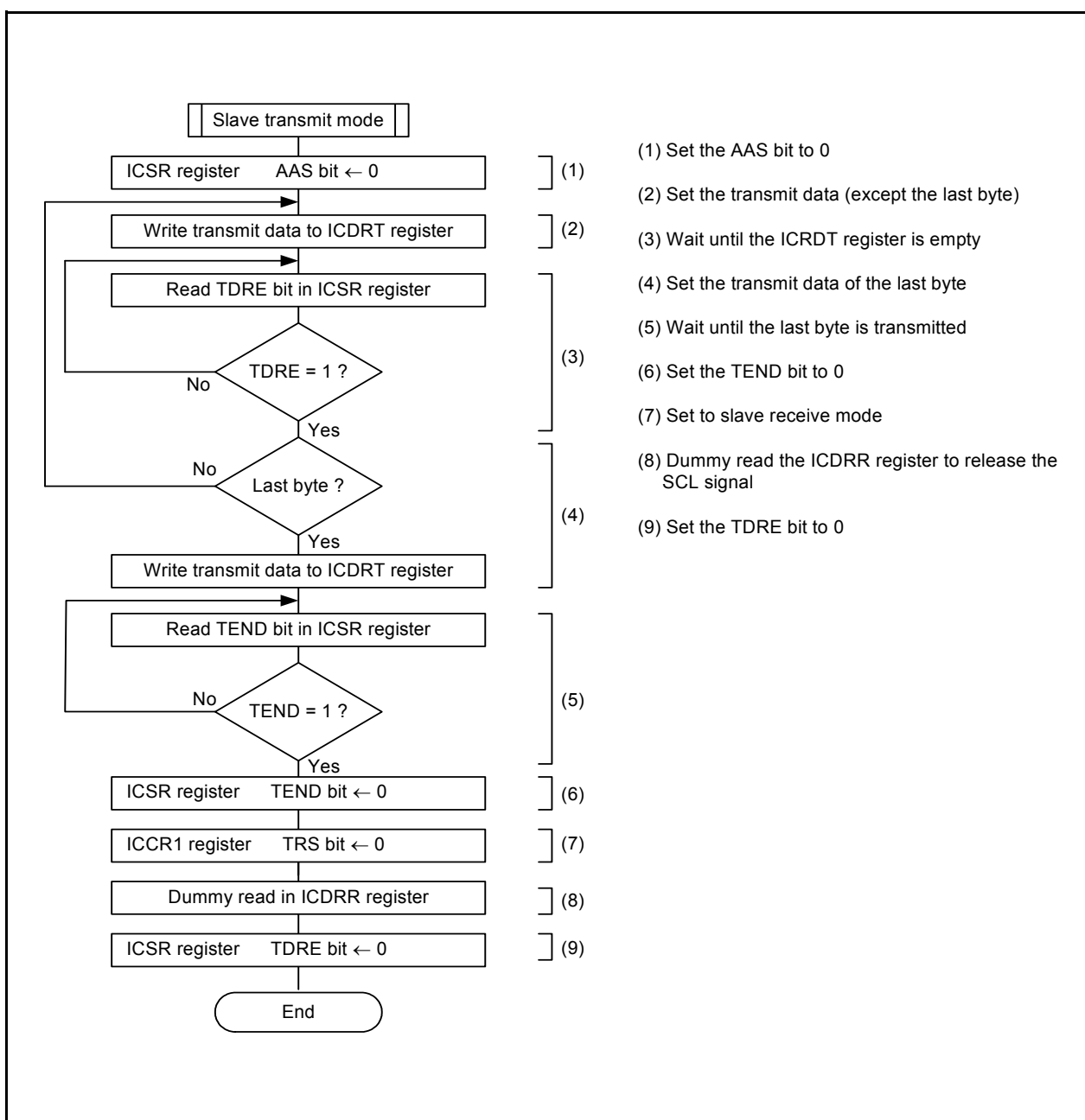
Figure 16.48 Example of Register Setting in Slave Transmit Mode (I²C bus Interface Mode)
