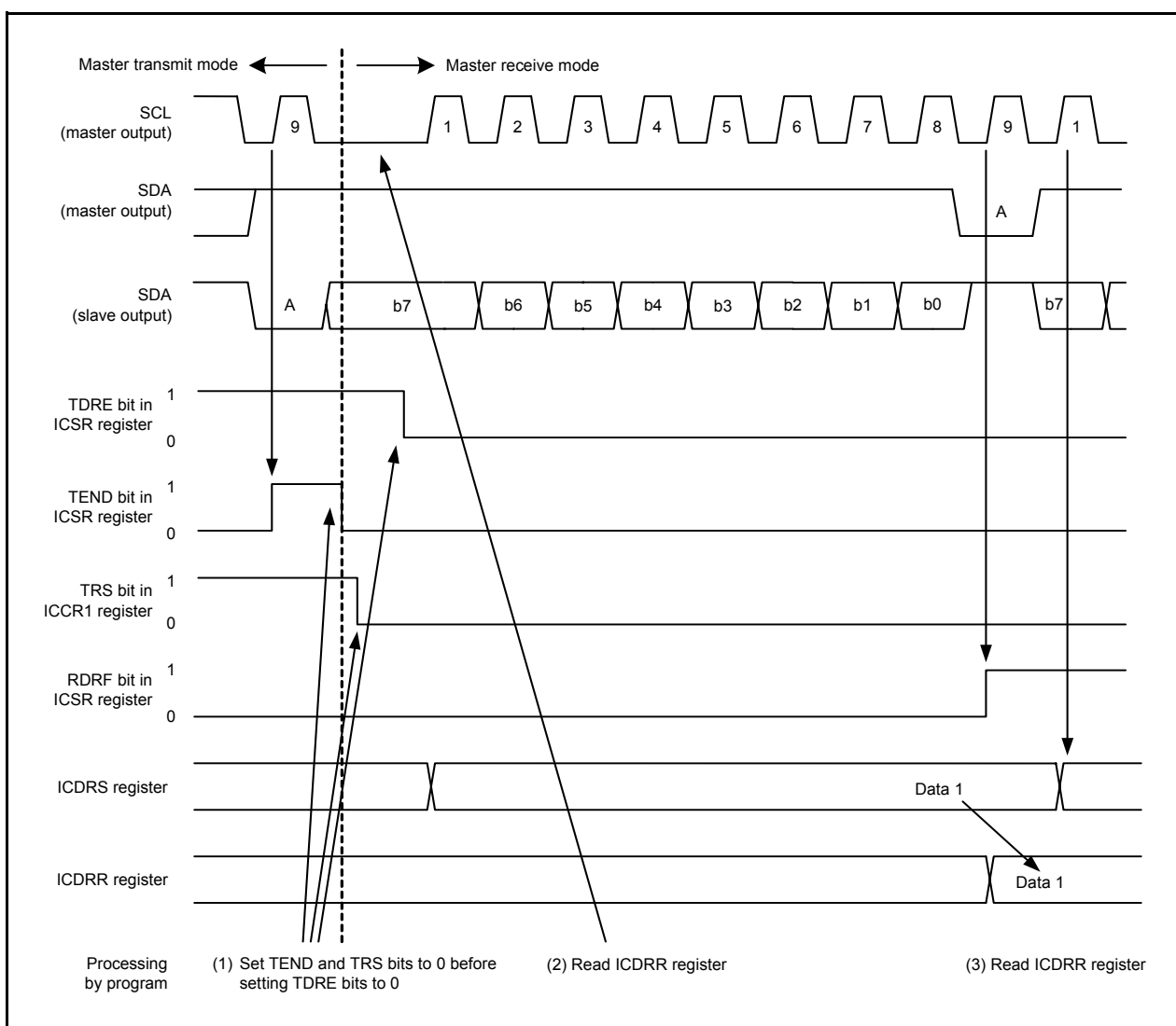
Figure 16.37 Operating Timing in Master Receive Mode (I²C bus Interface Mode) (1)
