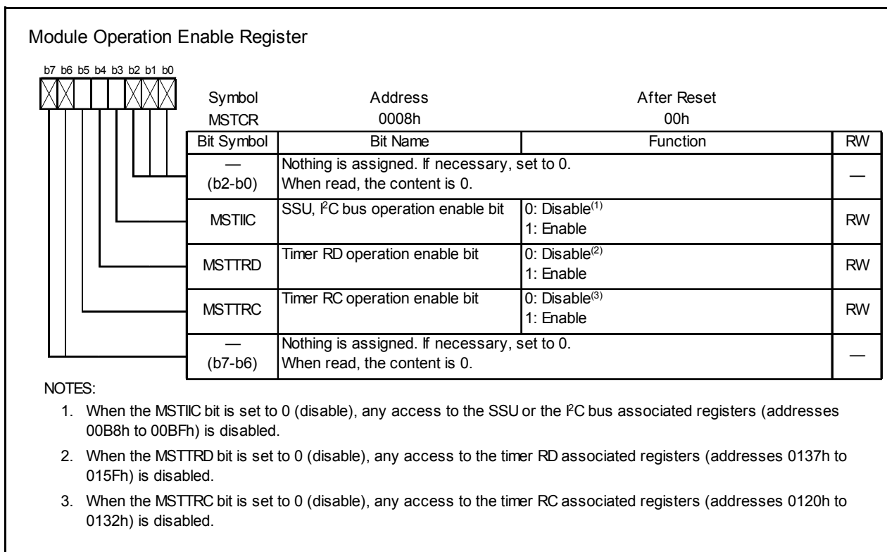
Figure 14.27 MSTCR Register
