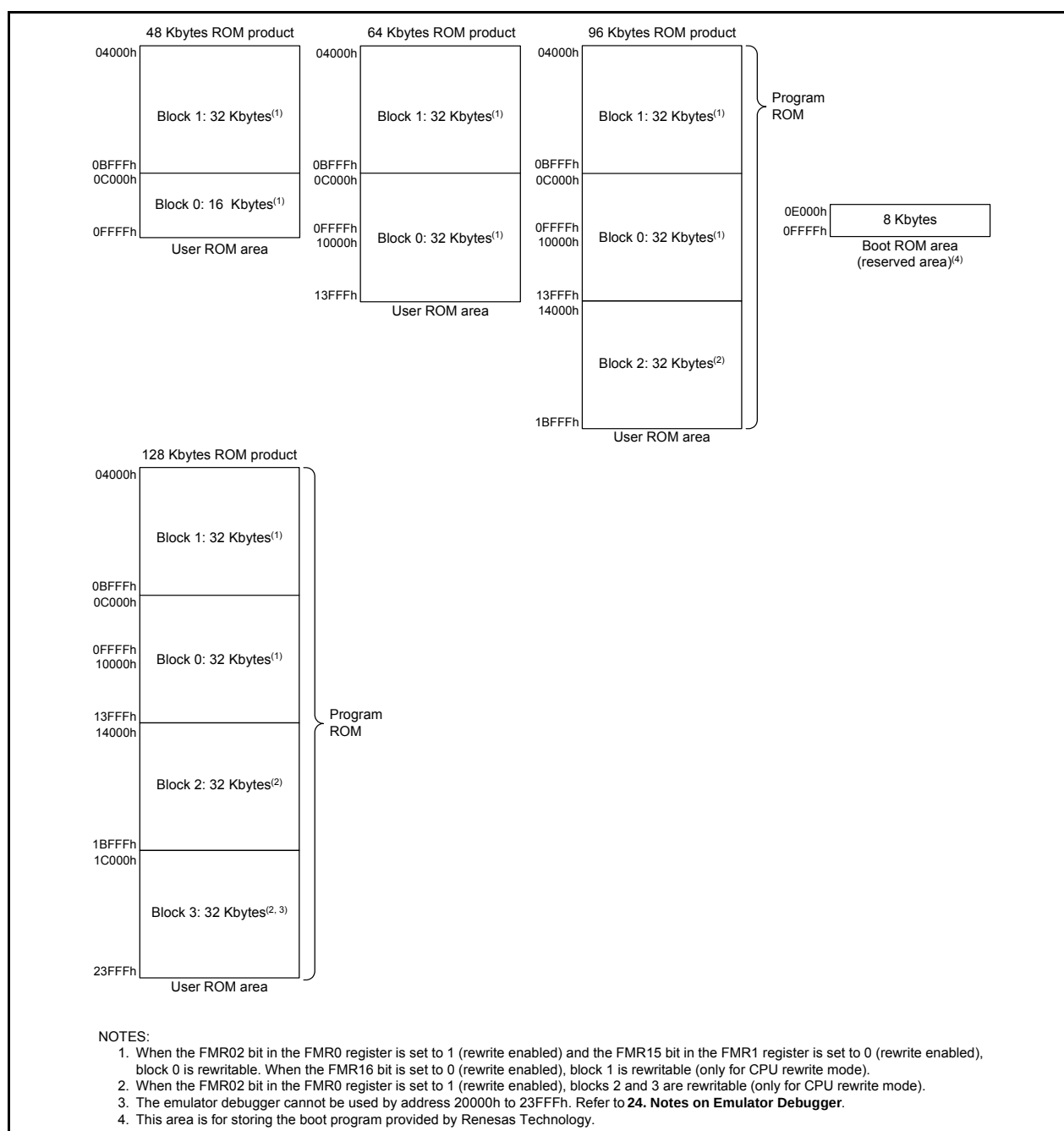
Figure 20.1 Flash Memory Block Diagram for R8C/2A Group
