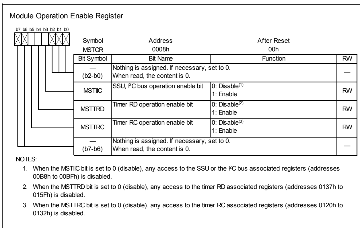
Figure 14.84 MSTCR Register
