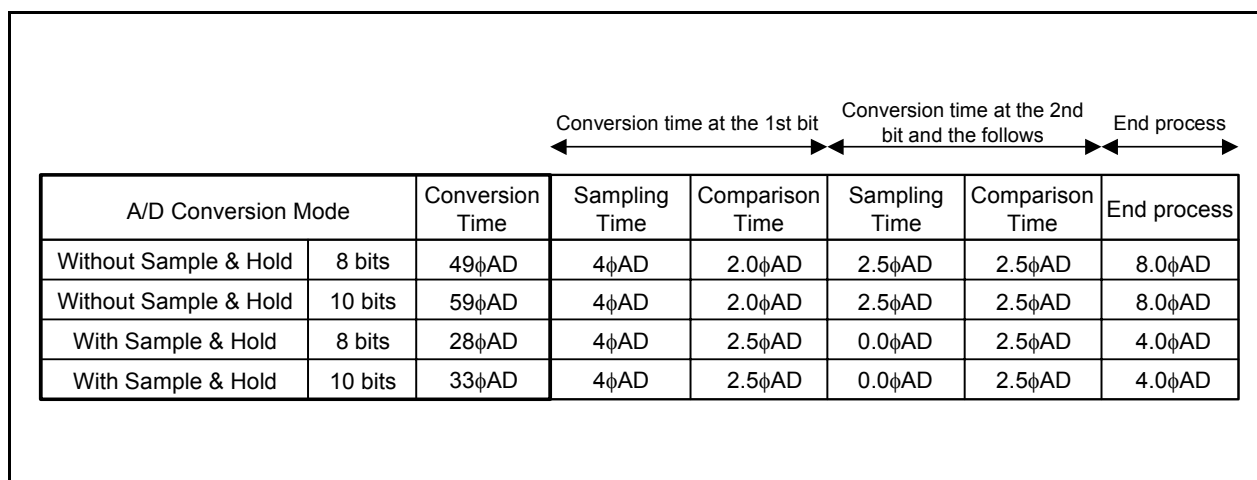
Figure 18.10 A/D Conversion Cycles
