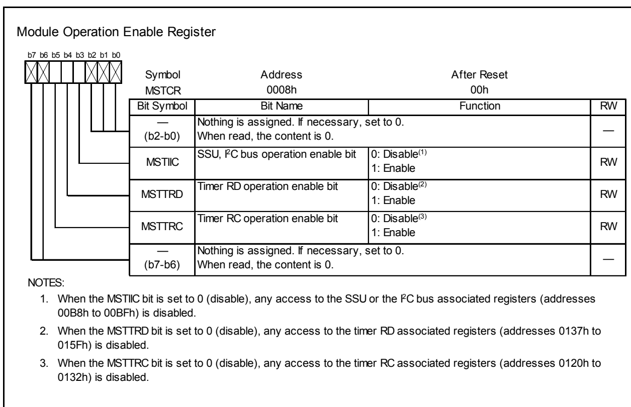
Figure 14.126 MSTCR Register
