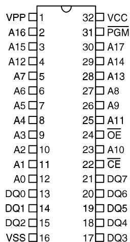
HT27C020 – 32 DIP/SOP
