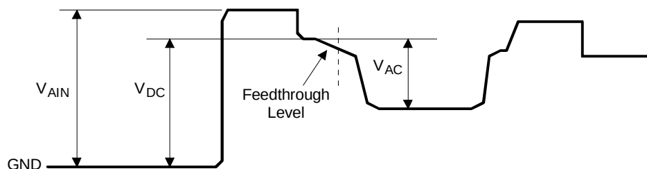
Figure 2. Analog Input
