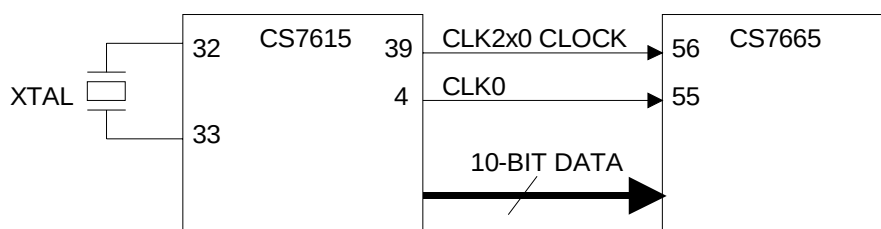
Figure 4. CS7615/CS7665 Interface
