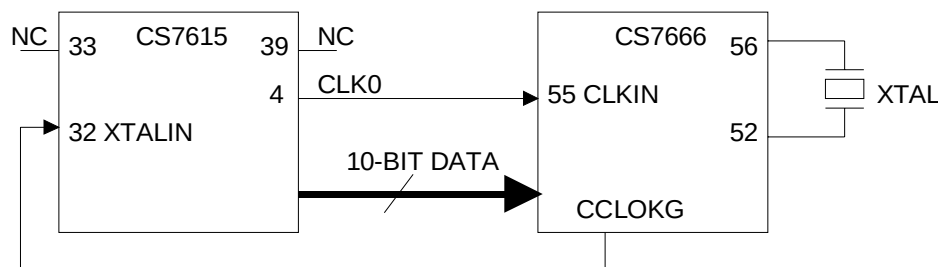
Figure 5. CS7615/CS7666 Interface
