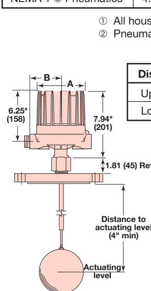
Model T20 with flange
