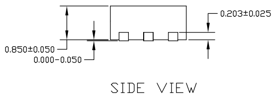
6-Pin 2mm x 2mm MLF ® (ML)
