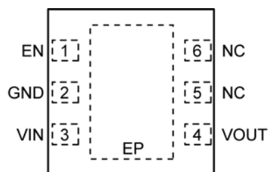
MIC5232-x.xYML 2mm x 2mm MLF® (ML)
