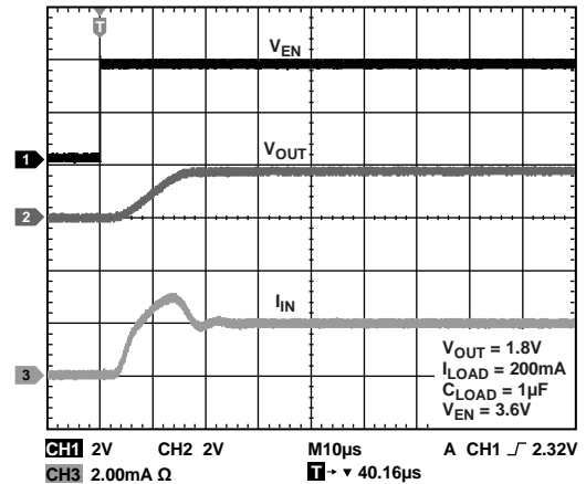
Figure 25. ADP190 Typical Rise Time and Inrush Current with C_{LOAD} = 1\mu\text{F}
