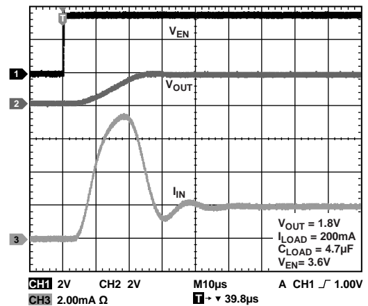
Figure 27. ADP190 Typical Rise Time and Inrush Current with C_{LOAD} = 4.7\mu\text{F}
