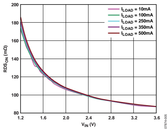
Figure 6. R_{DS\text{ON}} vs. Input Voltage, V_{IN} (Includes \sim 15\text{ m}\Omega Trace Resistance)
