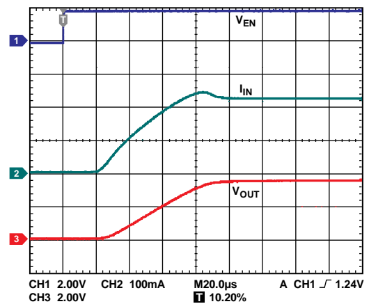
Figure 26. ADP191 Typical Rise Time and Inrush Current with C_{LOAD} = 1\mu\text{F}
