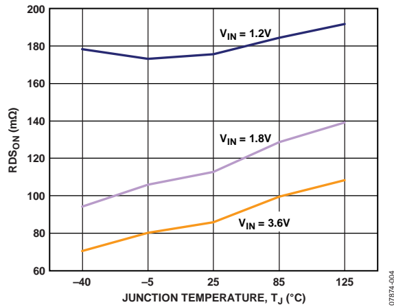
Figure 5. R_{DS\text{ON}} vs. Temperature (Includes \sim 15\text{ m}\Omega Trace Resistance)
