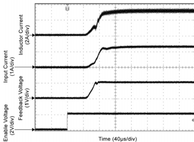
Start-Up Waveforms
