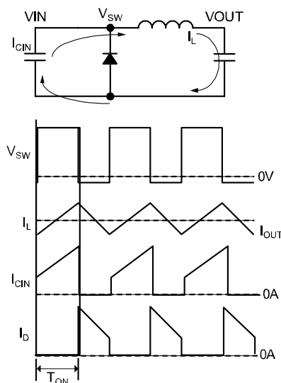
Figure 3. On-Time
