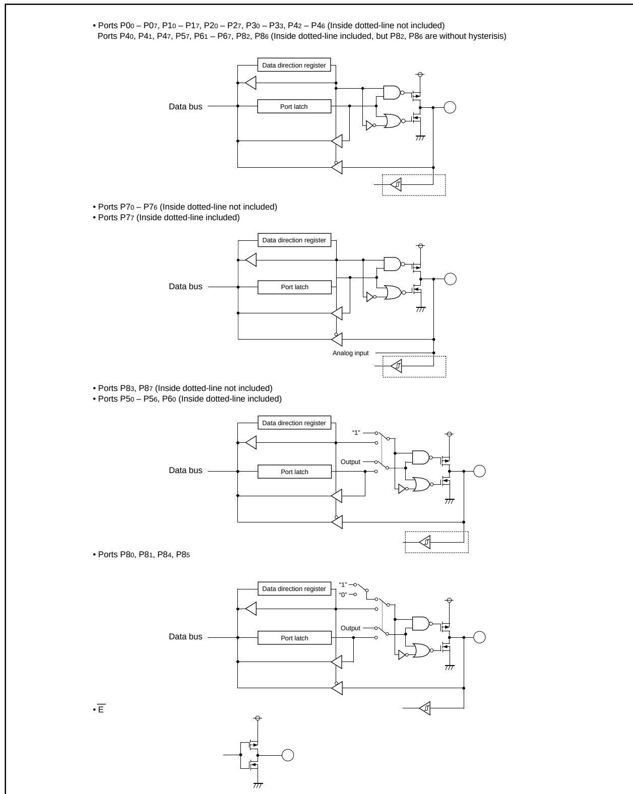
Fig. 50 Block diagram for ports P8 to P0 in single-chip mode and the \overline{E} pin output
