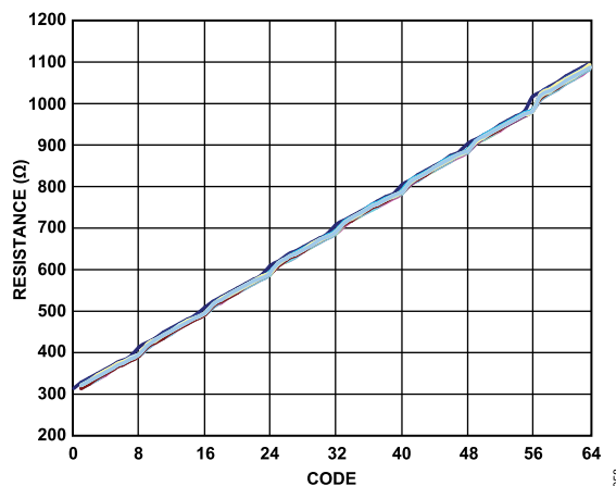
Figure 103. Typical CML Resistor Value vs. Register Code
