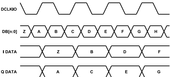
Figure 90. Timing Diagram with IFIRST = 0, IRISING = 1
