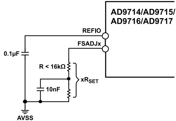
Figure 98. xR_{\text{SET}} Configuration for Values > 16 k \Omega
