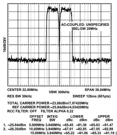
Figure 72. AD9717 Two-Carrier ACLR, 1.8 V
