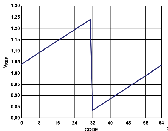
Figure 99. Typical V_{REF} Voltage vs. Code
