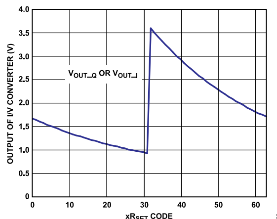
Figure 100. Effect of xR_{SET} Code
