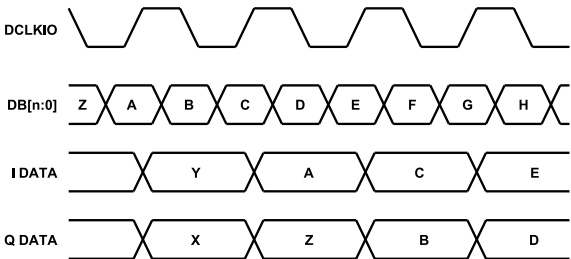
Figure 89. Timing Diagram with IFIRST = 0, IRISING = 0
