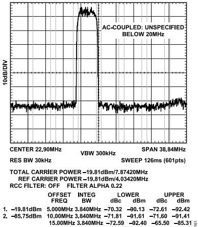
Figure 62. AD9717 One-Carrier ACLR, 1.8 V
