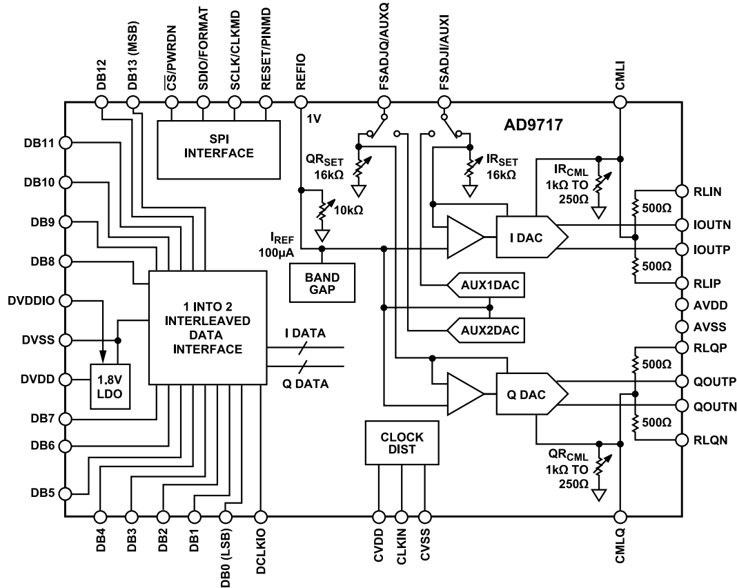
Figure 84. Simplified Block Diagram
