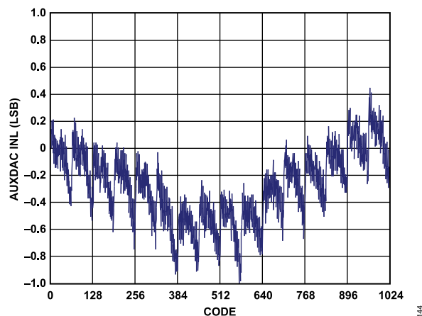
Figure 82. AUXDAC INL
