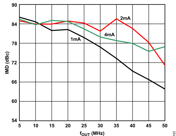
Figure 53. AD9717 IMD at Three Output Currents, 3.3 V
