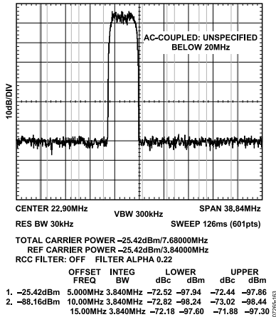
Figure 65. AD9717 One-Carrier ACLR, 3.3 V
