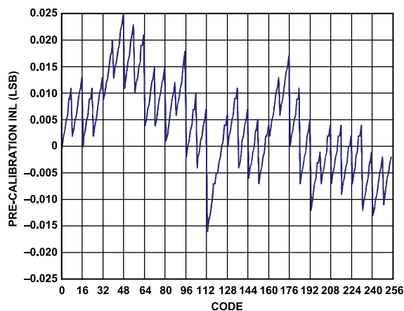
Figure 32. AD9714 Precalibration INL at 3.3 V
