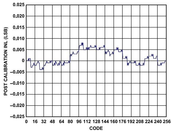
Figure 35. AD9714 Postcalibration INL at 3.3 V
