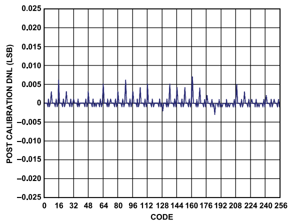
Figure 34. AD9714 Postcalibration DNL at 1.8 V
