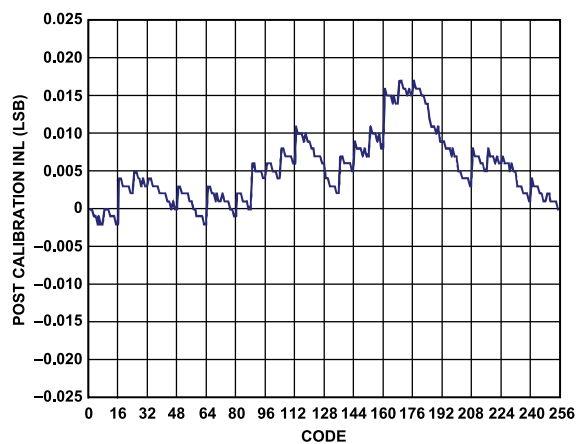
Figure 33. AD9714 Postcalibration INL at 1.8 V
