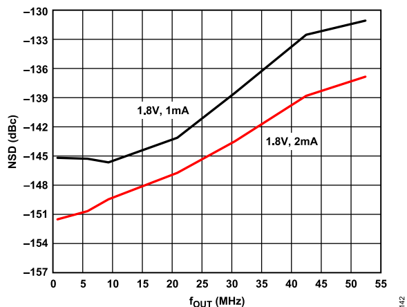
Figure 42. AD9717 Noise Spectral Density at Two Output Currents, 1.8 V
