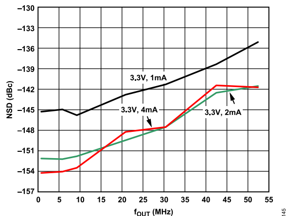
Figure 45. AD9717 Noise Spectral Density at Three Output Currents, 3.3 V
