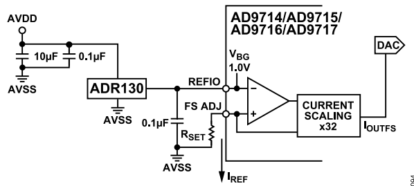
Figure 97. External Reference Configuration
