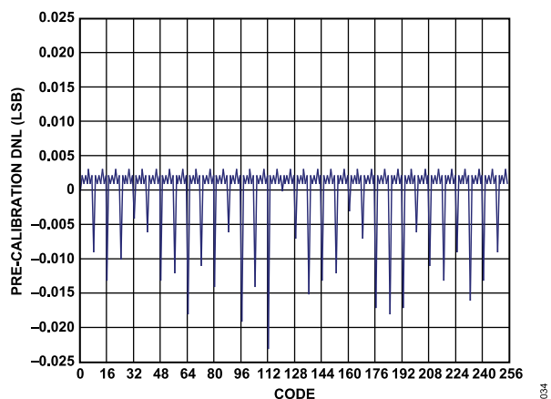
Figure 36. AD9714 Precalibration DNL at 3.3 V
