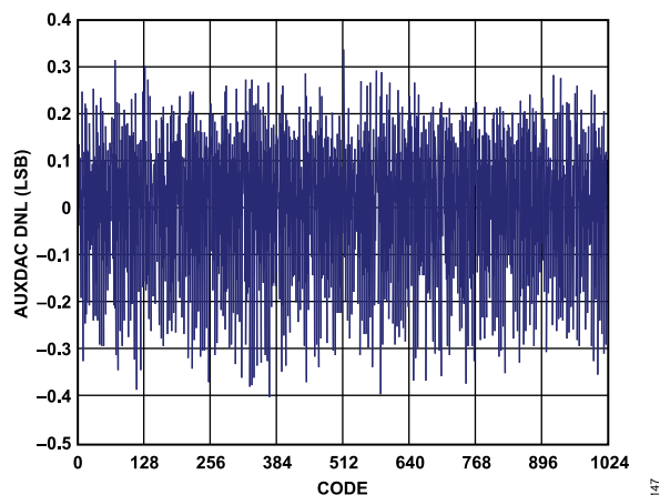
Figure 79. AUXDAC DNL
