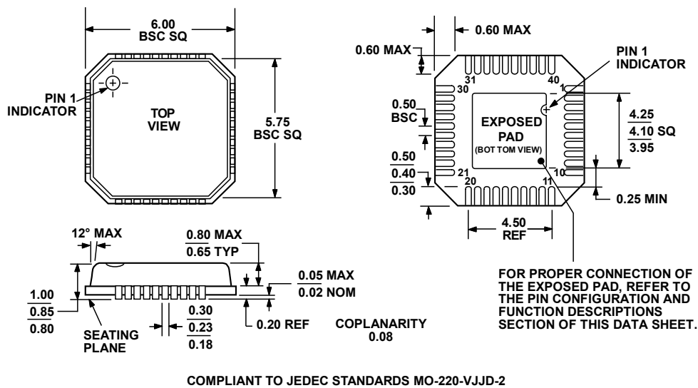
Figure 113. 40-Lead Lead Frame Chip Scale Package [LFCSP] 6 mm × 6 mm and 0.85 mm Package Height (CP-40-1) Dimensions shown in millimeters
