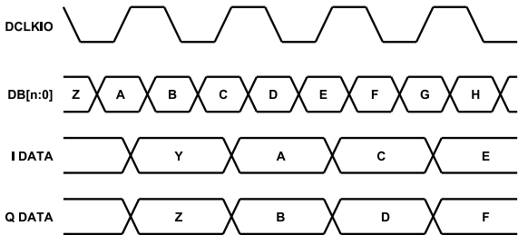
Figure 92. Timing Diagram with IFIRST = 1, IRISING = 1
