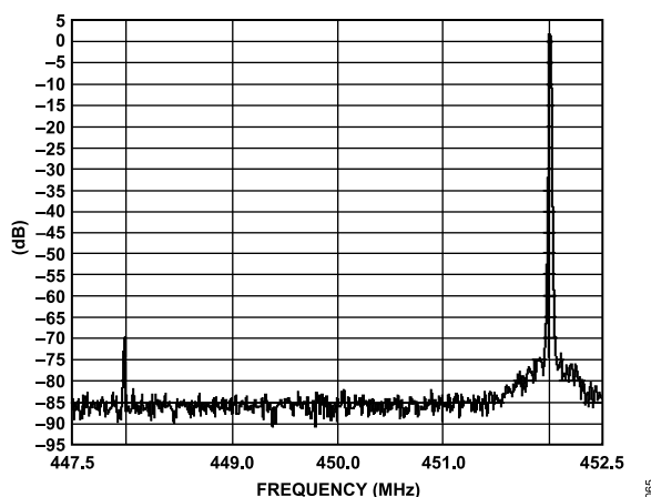
Figure 112. AD9714/AD9715/AD9716/AD9717 and ADL5370 with a Single-Tone Signal at 450 MHz, Gain and LO Compensation Optimized
