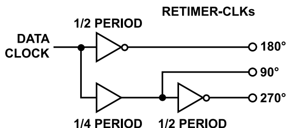
Figure 95. RETIMER-CLK Phases
