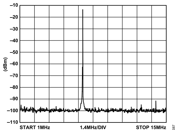
Figure 57. AD9717 Single-Tone Spectrum, 3.3 V
