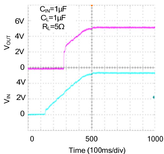
UVLO protection at rising
