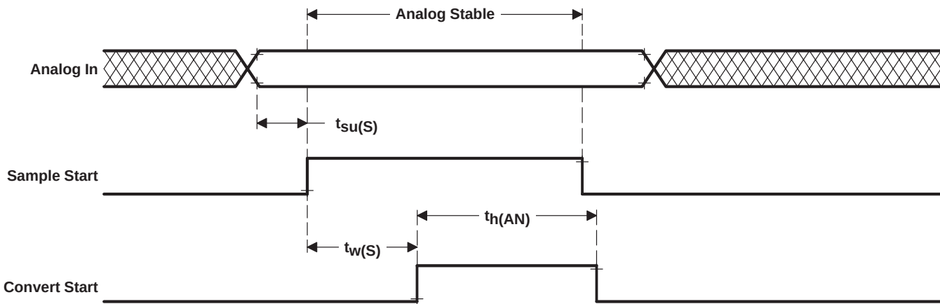
Figure 18. Analog Timing
