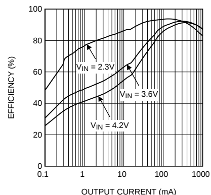
Figure 2. Efficiency vs. Output Current ( V_{OUT} = 1.8V , ECO Mode)
