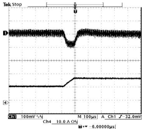
Vout= 3.3 V 50%-75% Load Transients at Vin=48 V
