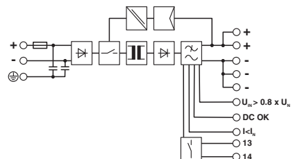
Block diagram
