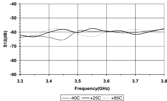
Narrowband S12 - Reverse Isolation
