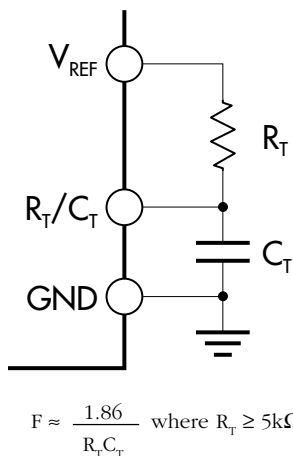
FIGURE 12 — OSCILLATOR TIMING CIRCUIT
