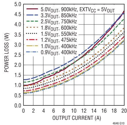
Figure 10. 8V IN Power Loss Curve
