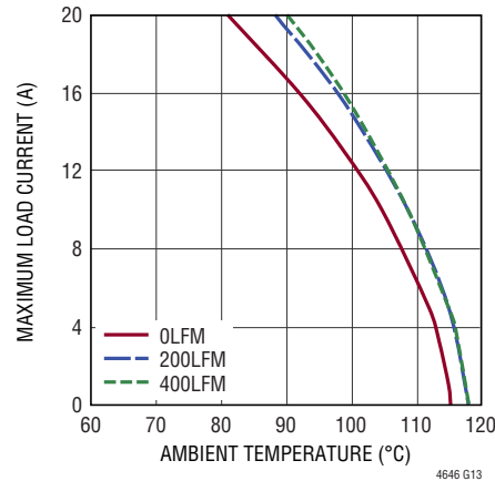
Figure 13. 12V to 1V Derating Curve, No Heat Sink, f_{SW} = 400\text{kHz}
