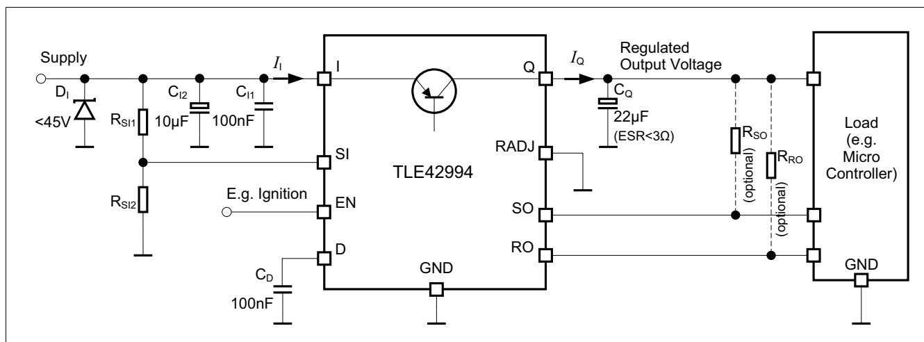
Figure 8 Application Diagram with Selecting Default Reset Thresholds
