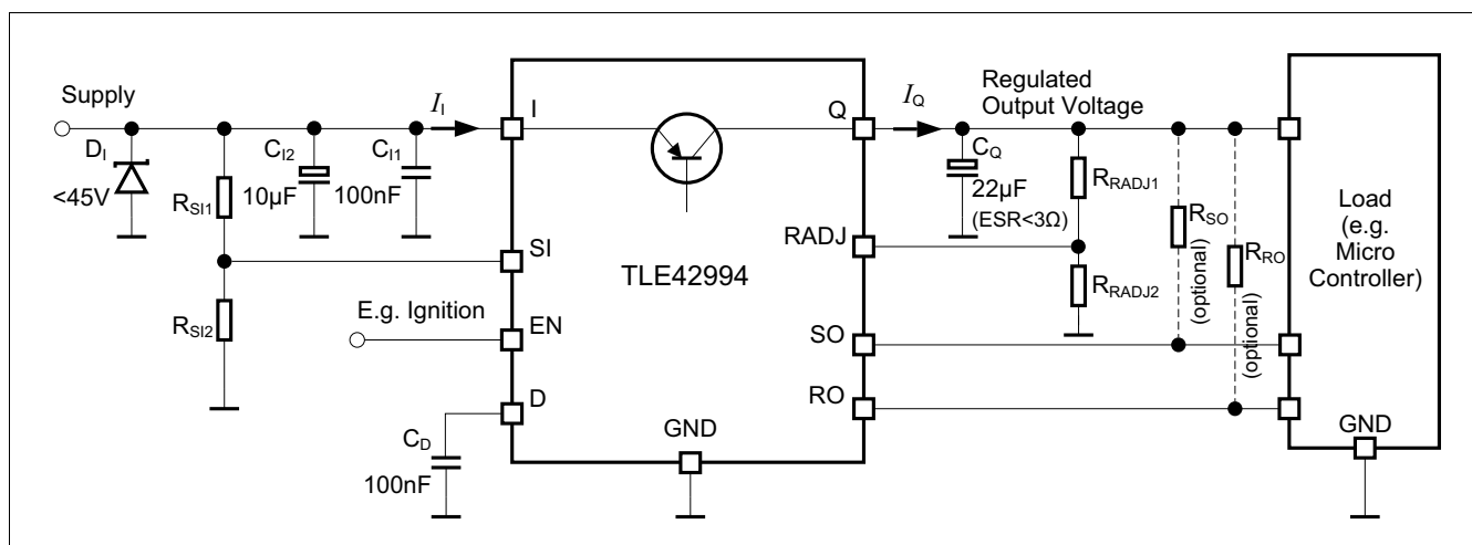
Figure 9 Application Diagram with Reset Thresholds Adjustment
