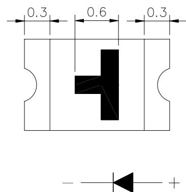
Recommend Pad Layout
