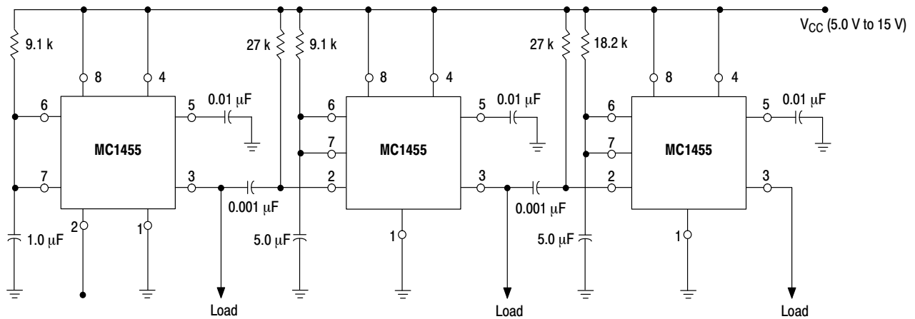
Figure 26. Sequential Timer
