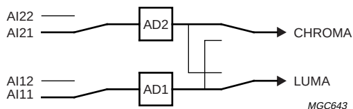
Fig.34 Mode 6 Y (automatic gain) + C (gain channel 2 adapted to Y gain).
