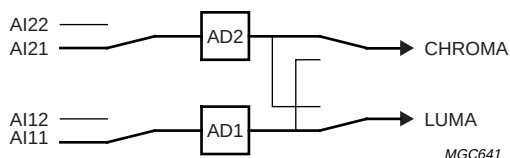
Fig.32 Mode 4 Y (automatic gain) + C (gain channel 2 fixed to GAI1 level).
