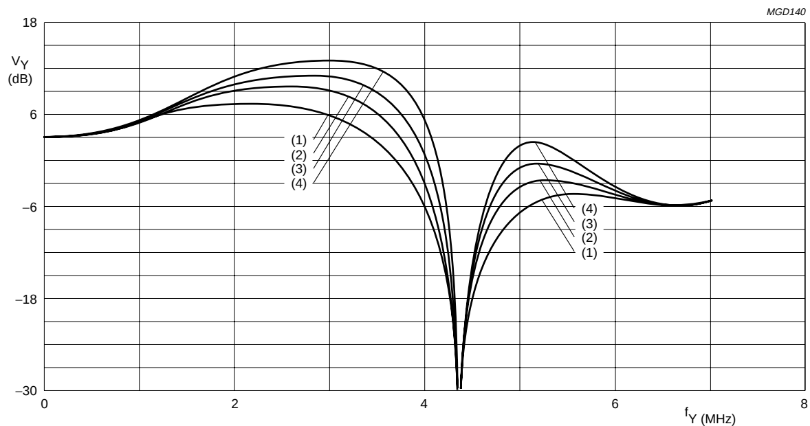
Fig.38 Luminance control SA 09H, 4.43 MHz Trap/CVBS mode, prefilter on and different aperture factors.
