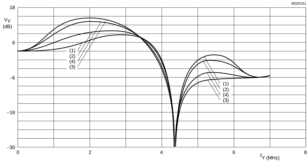
Fig.39 Luminance control SA 09H, 4.43 MHz Trap/CVBS mode, prefilter off and different aperture band-pass centre frequencies.
