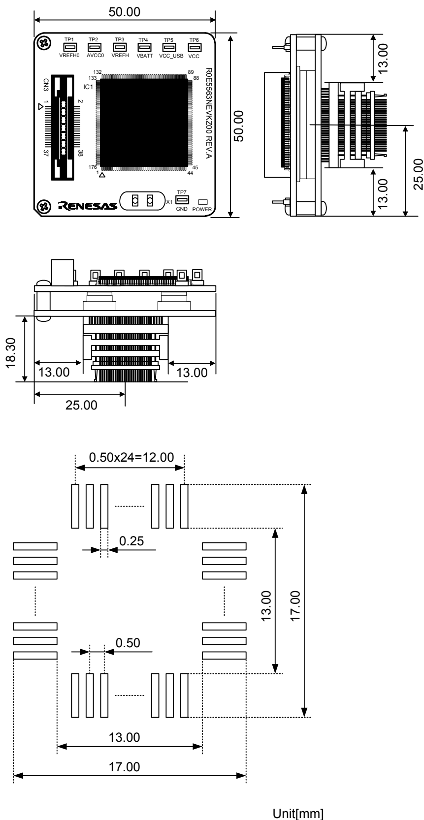
Figure 4 Reference Foot Pattern and Dimensions of This Product (R0E5563NEDMB01)
