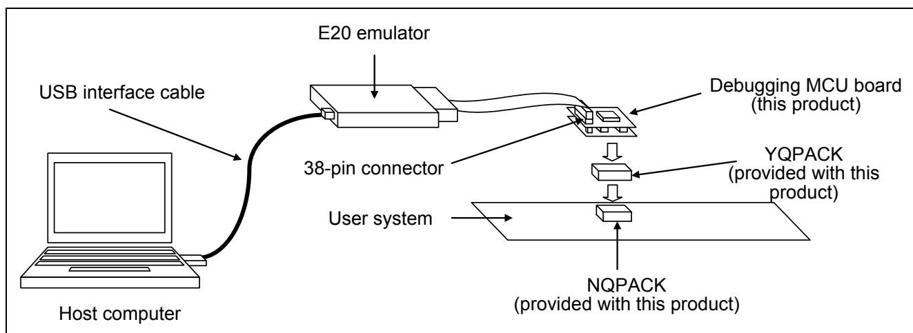
Figure 1 System Configuration
