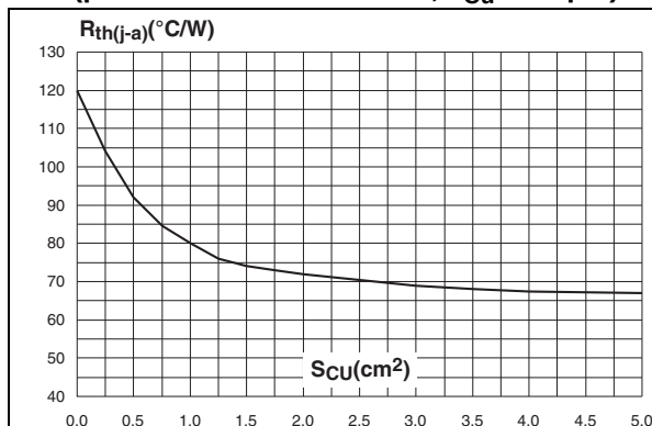
Figure 8. Thermal resistance junction to ambient versus copper surface under each lead (printed circuit board FR4, e_{Cu} = 35 \mu\text{m} )
