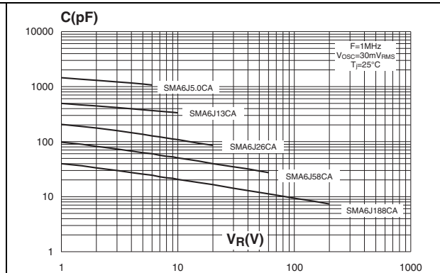
Figure 5. Junction capacitance versus reverse applied voltage (typical values) (SMA6JxxCA)
