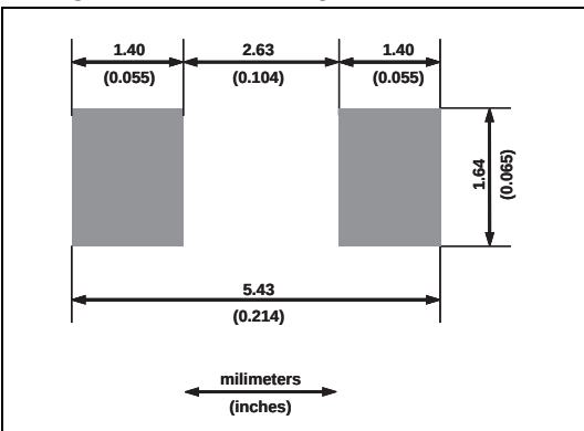
Figure 11. SMA footprint dimensions
