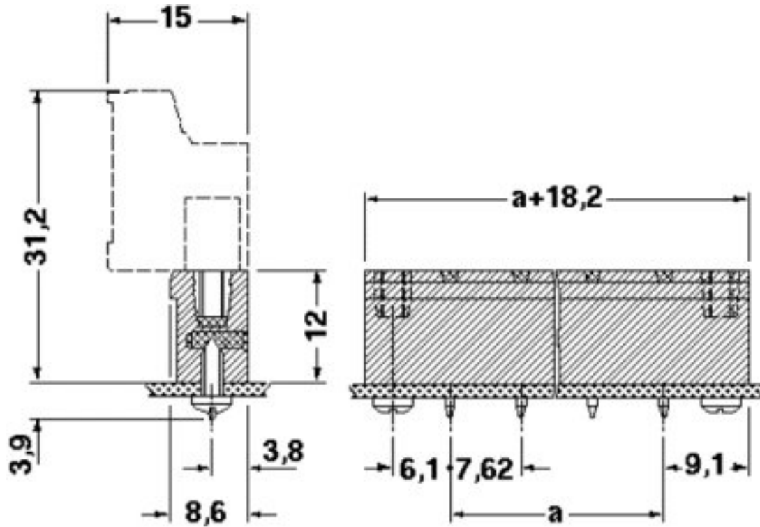
Dimensioned drawing
