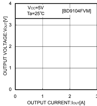
Fig.8 I OUT -V OUT
