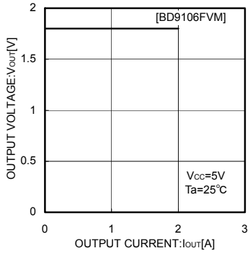
Fig.9 I OUT -V OUT
