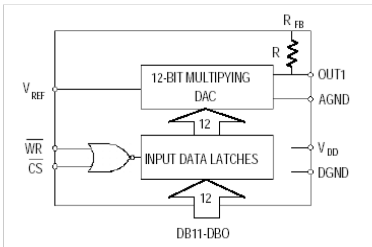
BLOCK DIAGRAM
