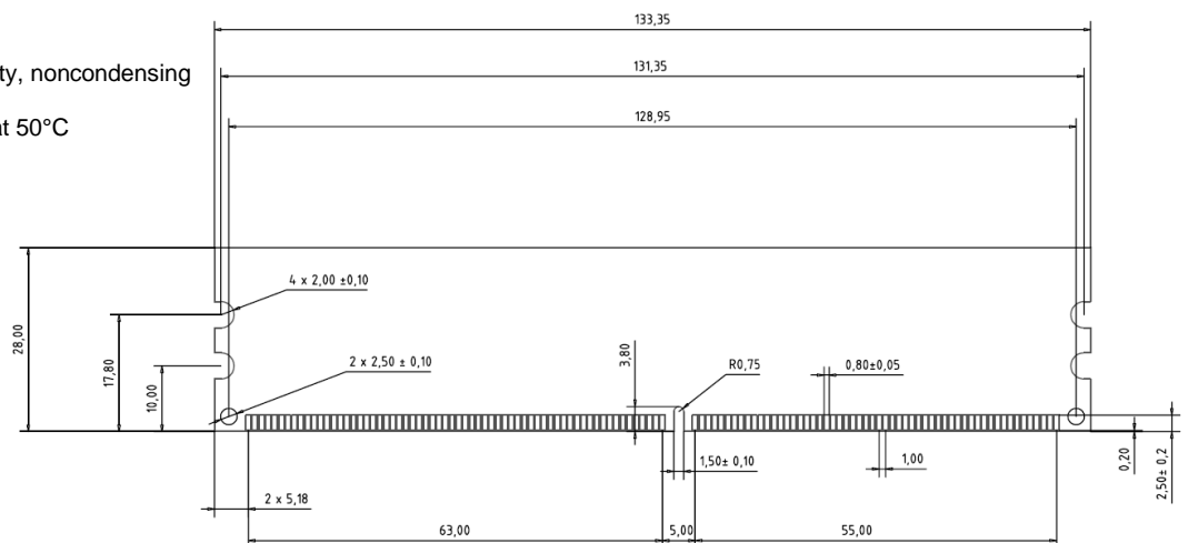
Figure: mechanical dimensions 1
