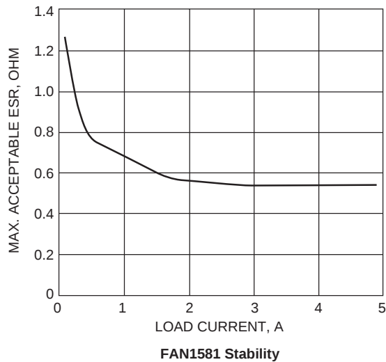
FAN1581 Stability
