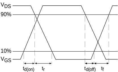
Fig 26b. Switching Time Waveforms
