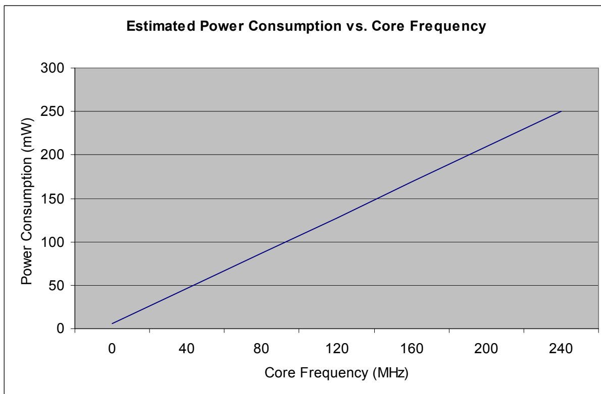
Figure 9. Estimated Maximum RUN Mode Power Consumption
