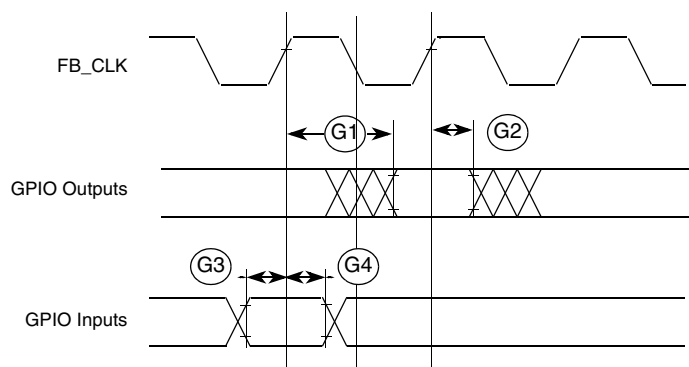
Figure 18. GPIO Timing
