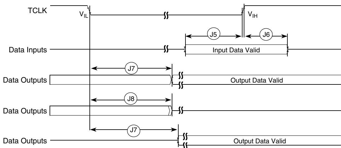
Figure 28. Boundary Scan (JTAG) Timing
