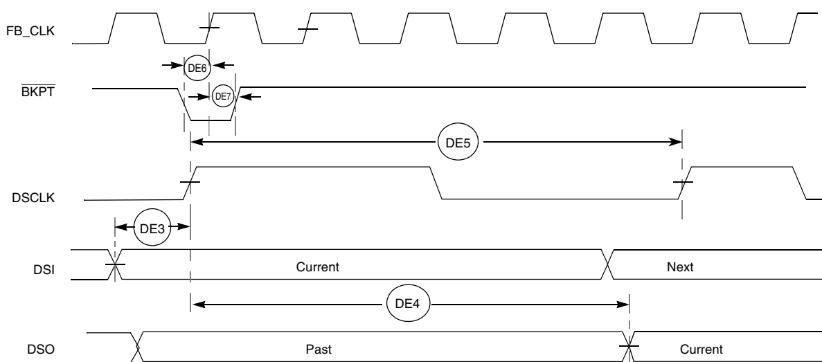
Figure 32. BDM Serial Port AC Timing
