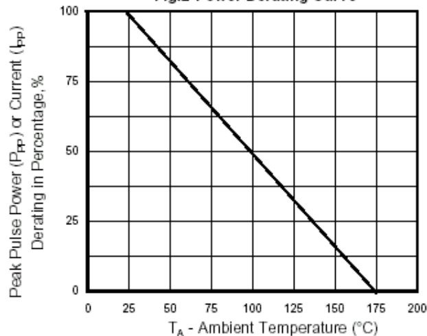
Fig.2-Power Derating Curve
