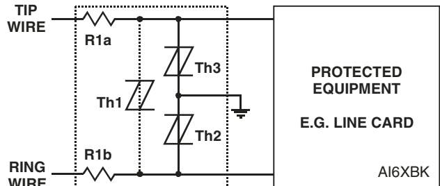
Figure 15. Protection Module
