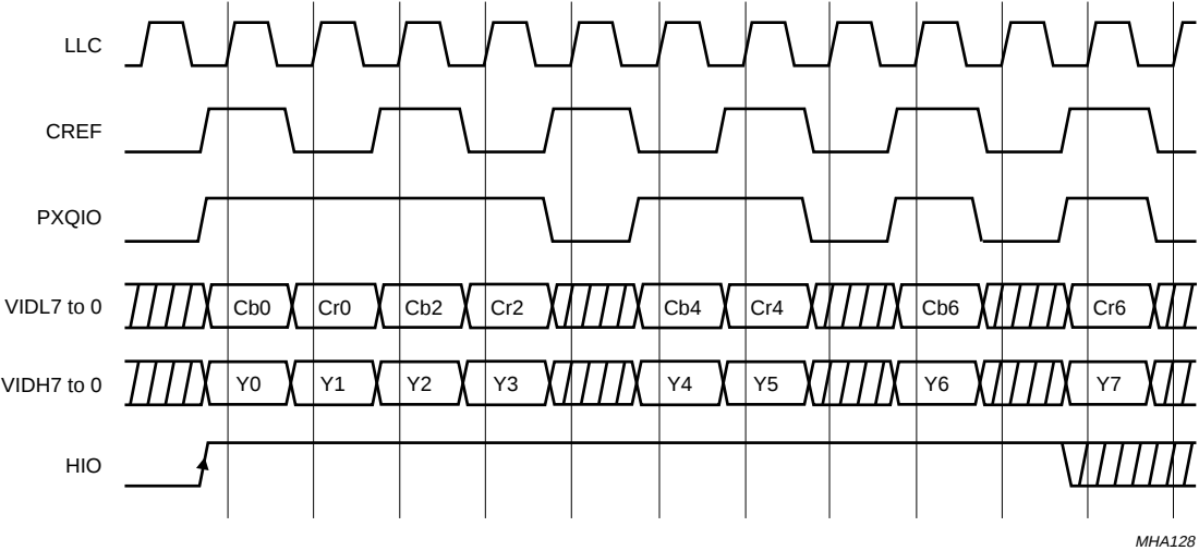
Fig.10 Timing of PXQIN for zoomed 16-bit data output at expansion port.
