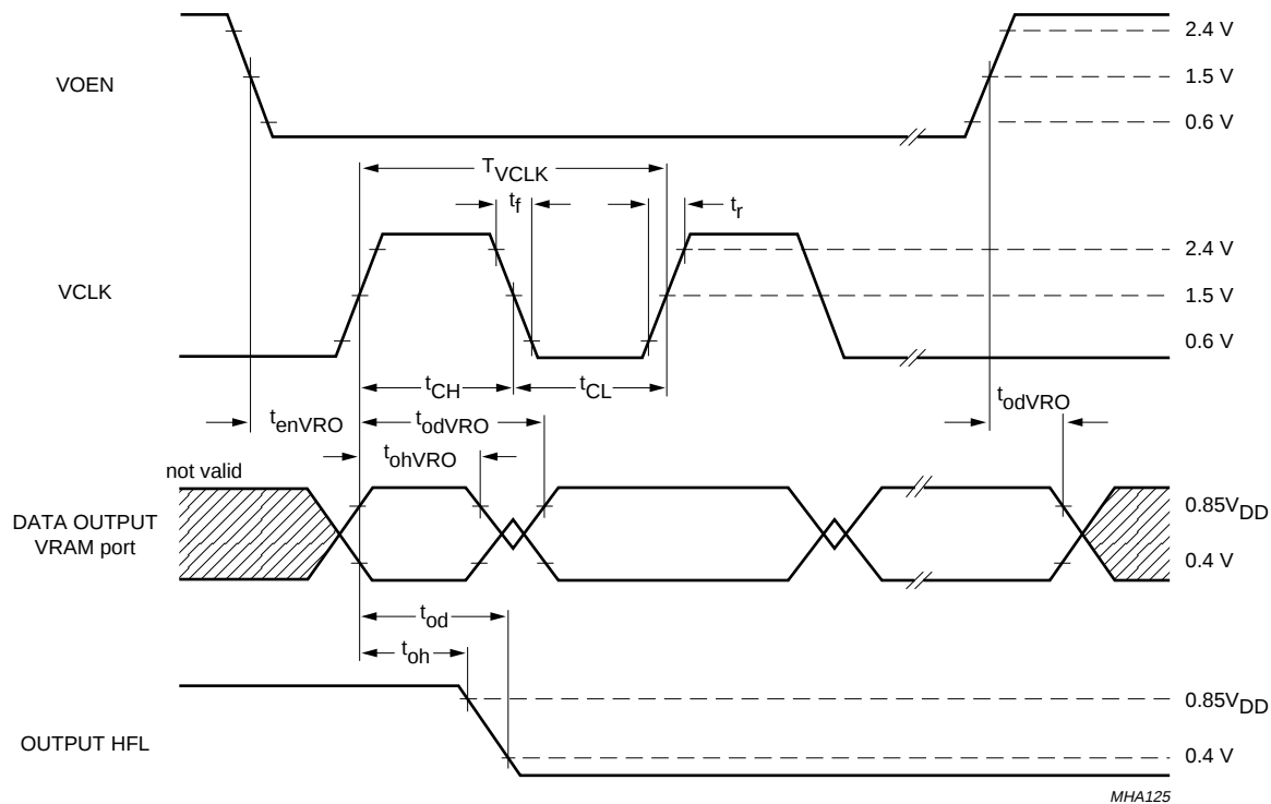
Fig.19 Data output timing (VRAM port).
