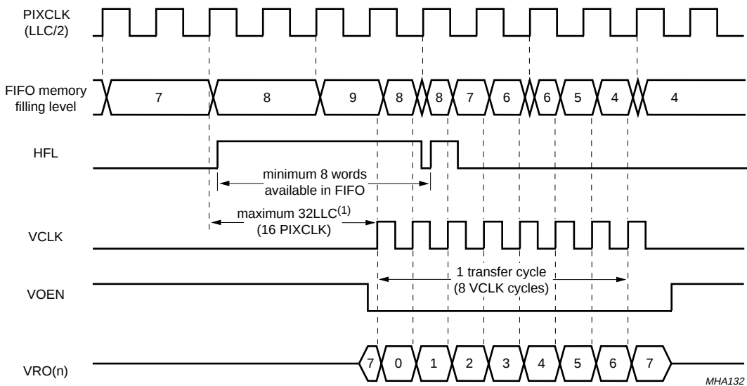
If VCLK cycles occur at VOEN = HIGH the FIFO register is unchanged but the outputs VRO31 to VRO0 remain in the 3-state position. (1) Only valid for non-zoomed data.
