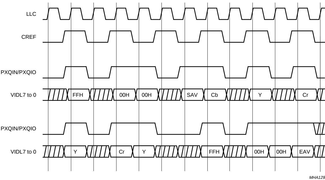
Fig.8 Timing of PXQIN/PXQIO for CCIR 656 data input at expansion port.
