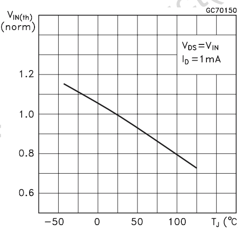
Figure 12. Normalized Input Threshold Voltage vs Temperature
