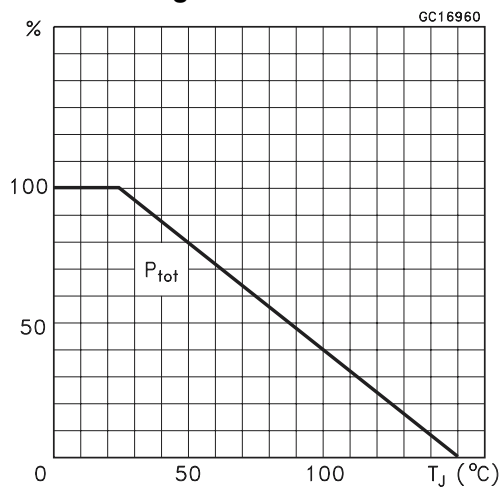
Figure 4. Derating Curve
