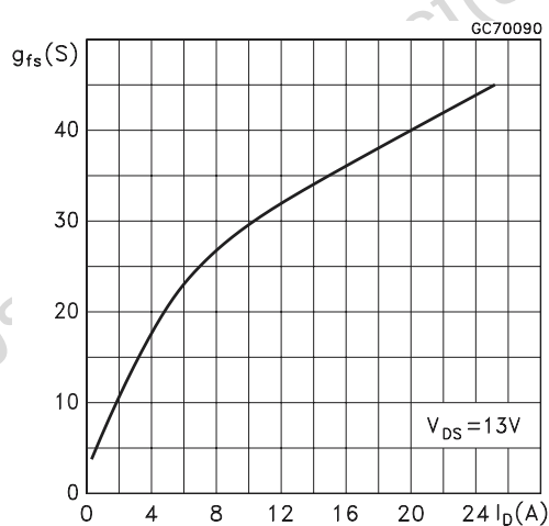
Figure 6. Transconductance
