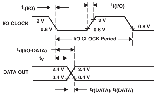
Figure 6. I/O CLOCK and DATA OUT Voltage Waveforms
