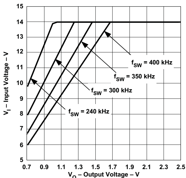
Figure 26. V_O Ripple Regions
