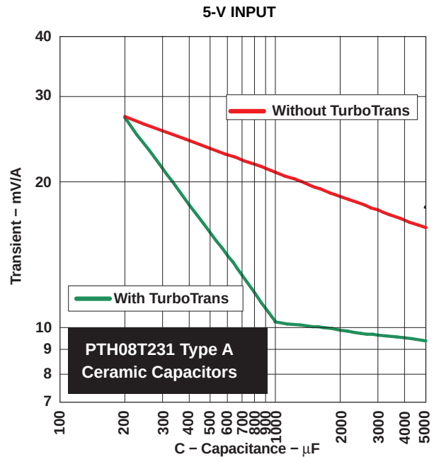
Figure 13. Capacitor Type A, 100 \leq C(\mu F) \times ESR(m\Omega) \leq 1000 (e.g. Ceramic)
