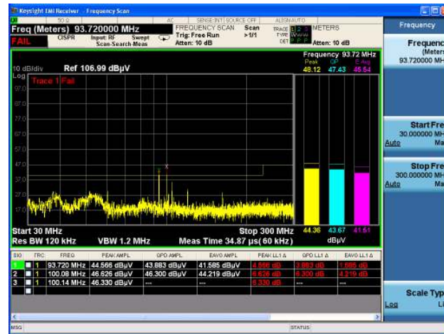
Figure 1. Frequency scan
