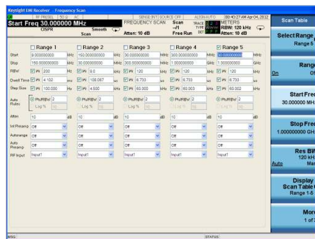
Figure 3. Scan table
