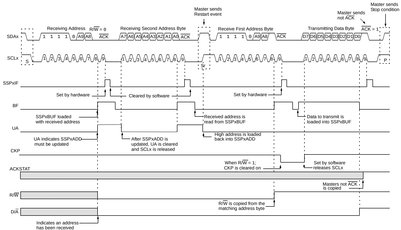
FIGURE 15-22: I 2 C SLAVE, 10-BIT ADDRESS, TRANSMISSION (SEN = 0, AHEN = 0, DHEN = 0)
