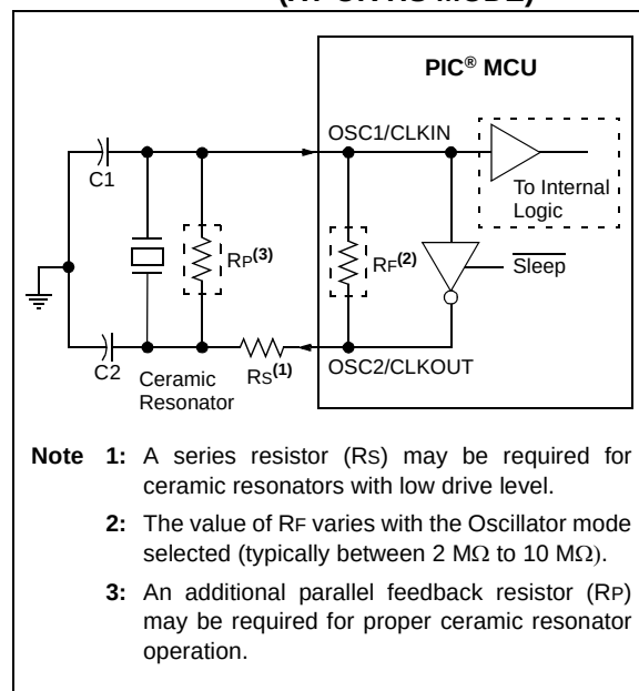
FIGURE 2-7: CERAMIC RESONATOR OPERATION (XT OR HS MODE)
