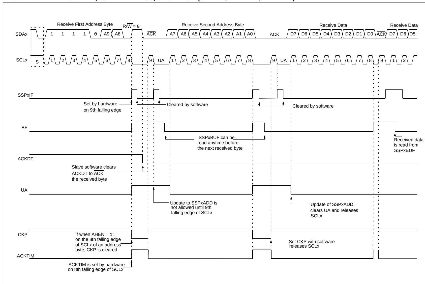
FIGURE 15-21: I 2 C SLAVE, 10-BIT ADDRESS, RECEPTION (SEN = 0, AHEN = 1, DHEN = 0)
