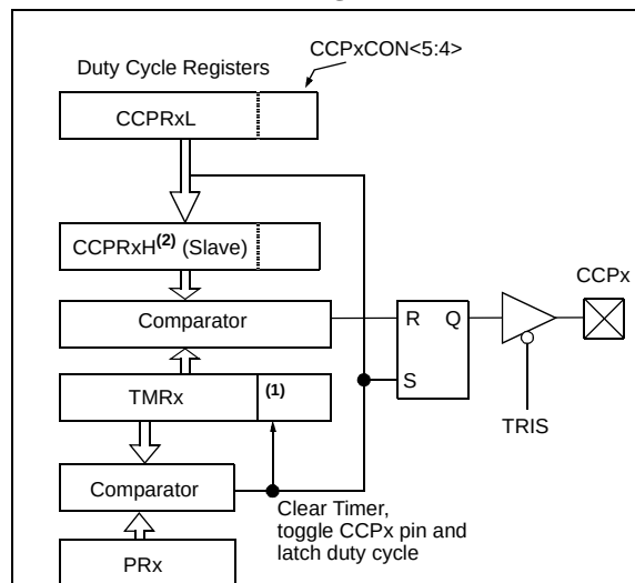
FIGURE 14-4: SIMPLIFIED PWM BLOCK DIAGRAM
