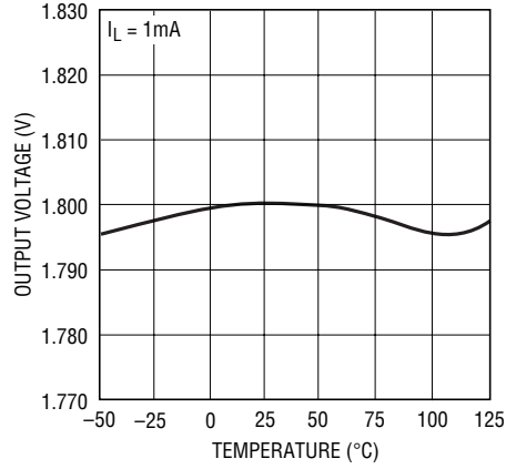
Output Voltage
