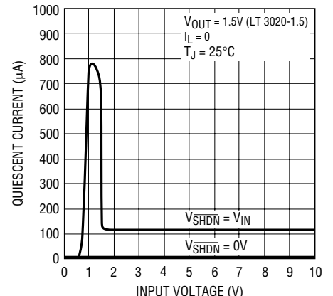
Quiescent Current
