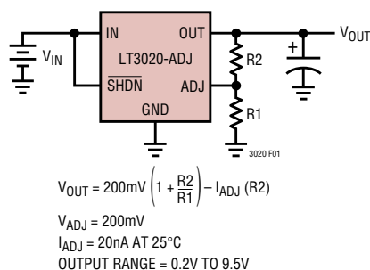
Figure 1. Adjustable Operation
