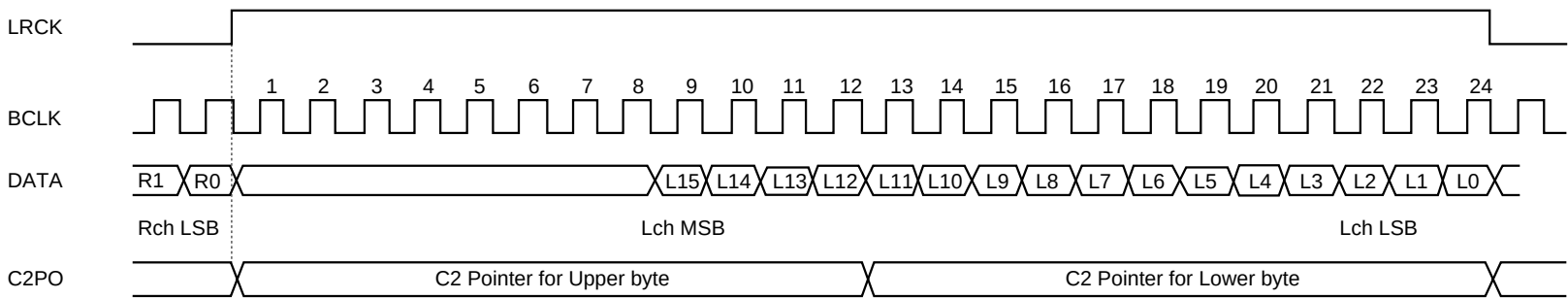
Fig. 2.1.1 (3) CXD2500Q, 48 bit Slot Mode Timing Chart
