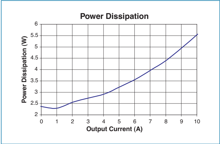
Figure 4 — Example power dissipation vs. output current. (MT036A120M010FP)
