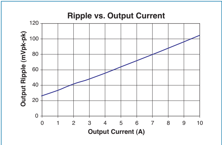
Figure 2 — Sample output voltage ripple vs. output current with no POL bypass capacitance. (MT036A120M010FP)
