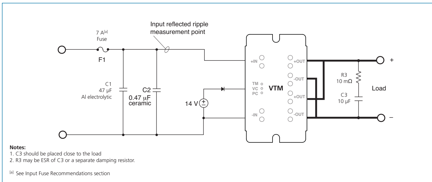
Figure 10 — VI BRICK VTM test circuit
