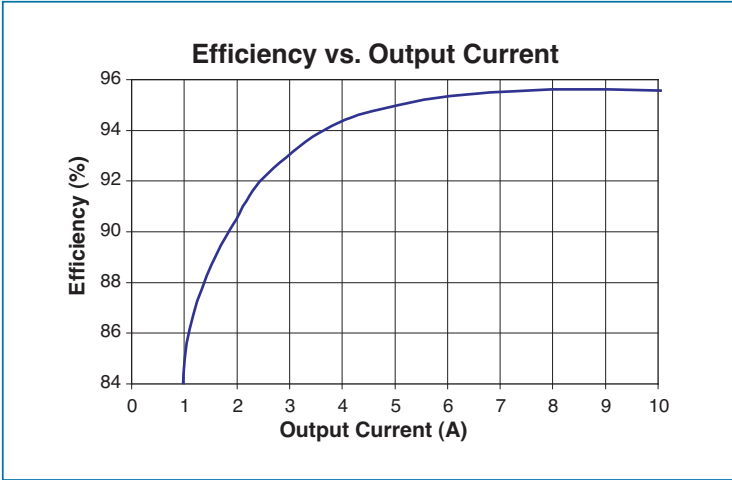
Figure 3 — Representative efficiency vs. output current. (MT036A120M010FP)
