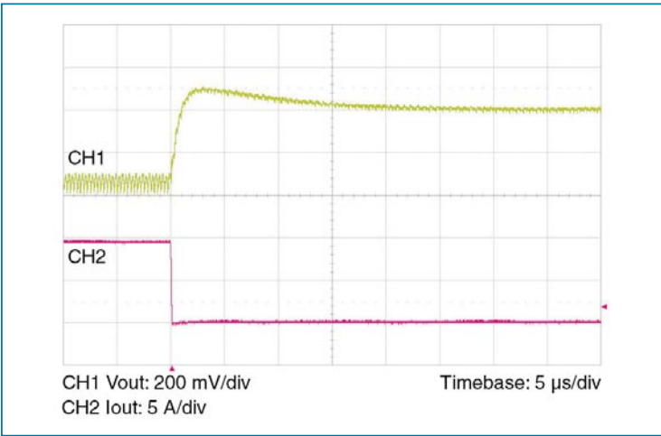
Figure 8 — Example load step with 100 \mu F input capacitance and no output capacitance. (MT036A120M010FP)
