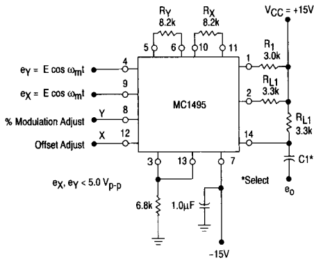
Figure 30. Amplitude Modulation
