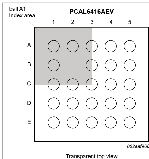
Figure 4. Pin configuration for VFBGA24 (3 mm × 3 mm)
