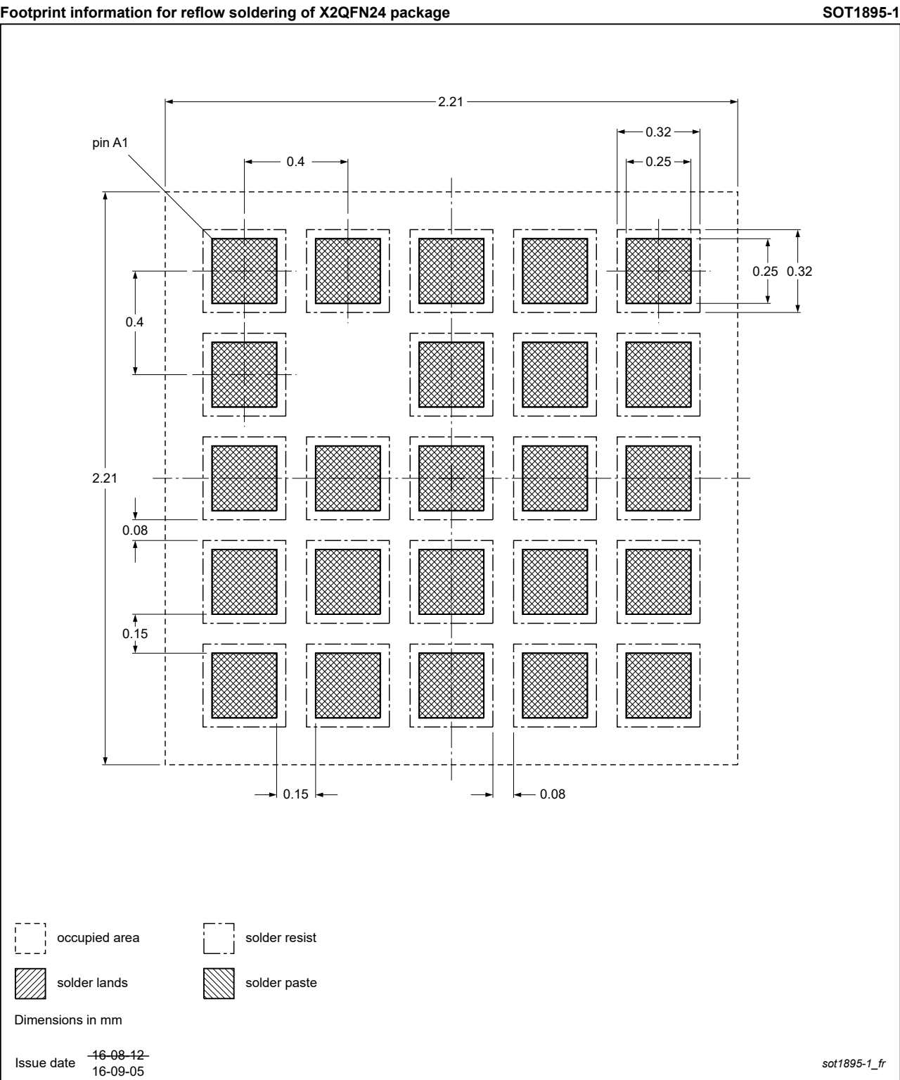
Figure 45. PCB footprint for SOT1895-1 (X2QFN24); reflow soldering
