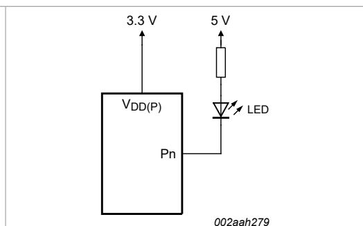
Figure 19. Device supplied by a lower voltage
