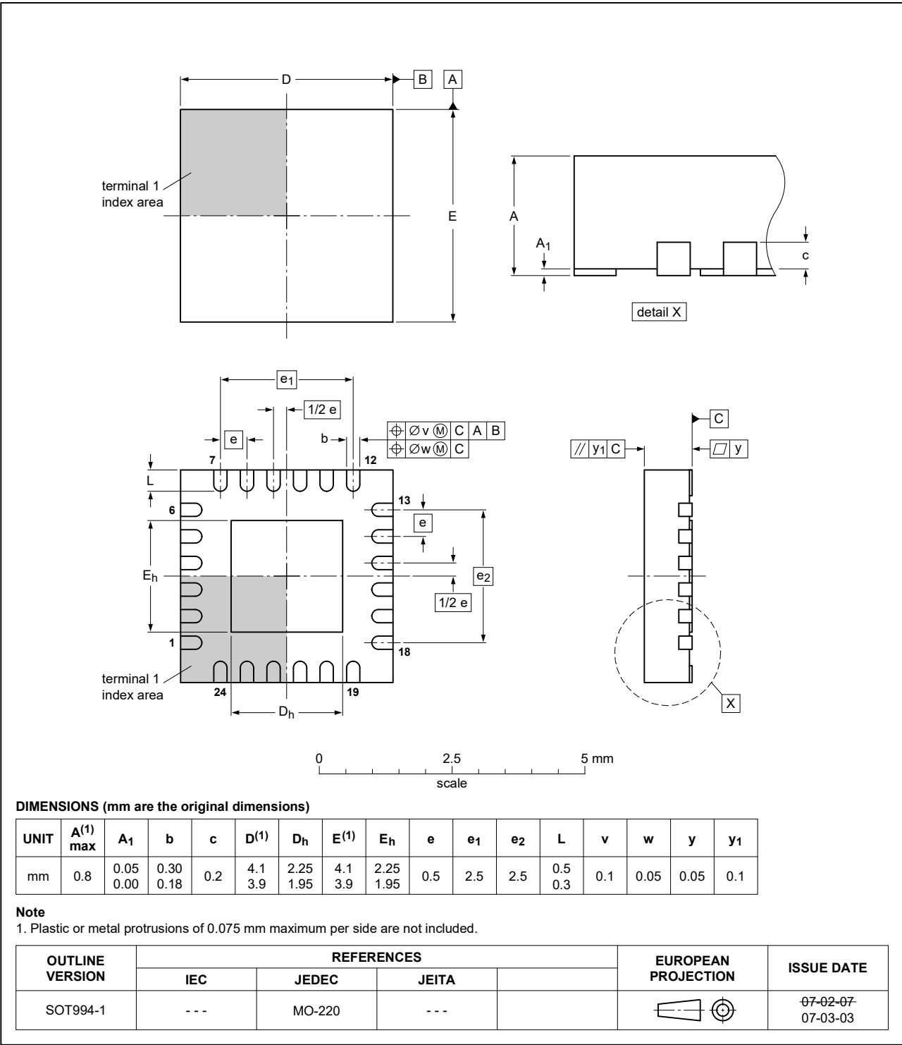
Figure 37. Package outline SOT994-1 (HWQFN24)
