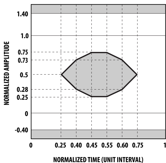
Figure 5b. Transmitter Optical Eye Mask Definition
