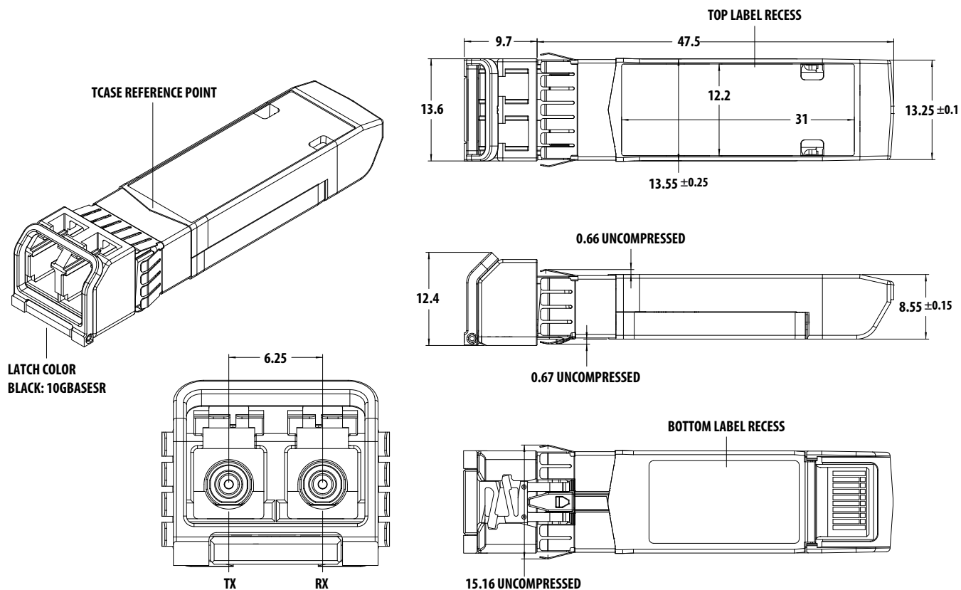
Figure 7. Module drawing
