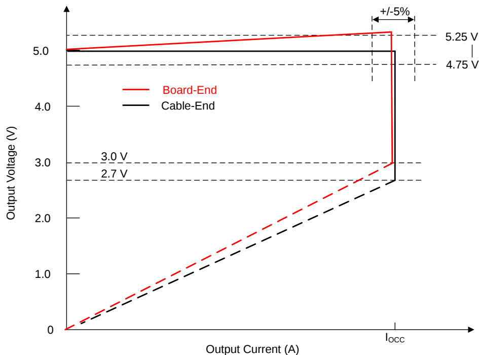
图 21. Typical Target Output V-I Curves
