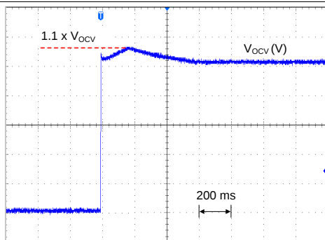
图 30. Typical V_{OUT} Start Up at No Load
